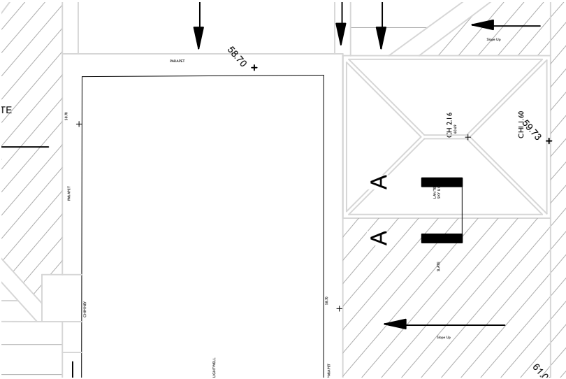
2 Roof Plan Scale: 1:100
