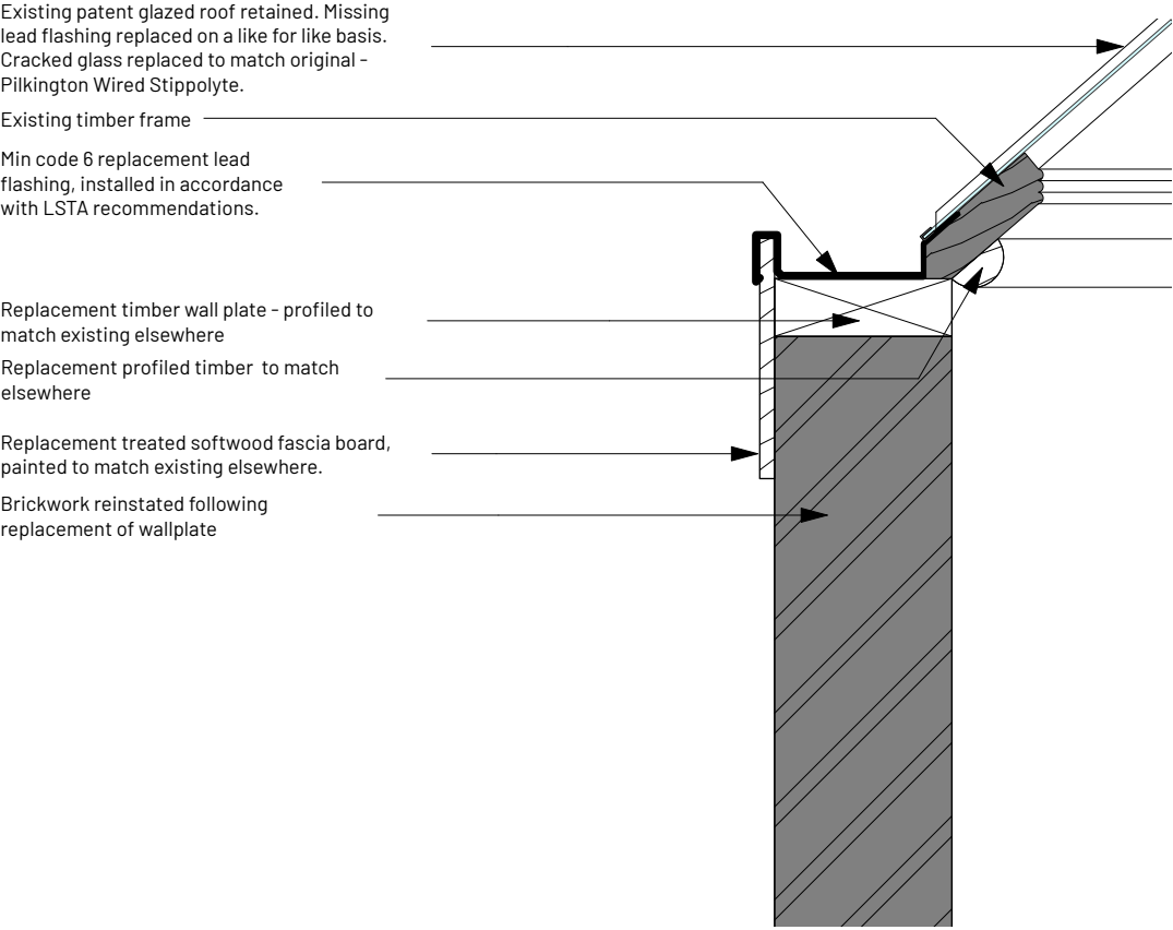
1 Detail - Existing lantern roof repairs Section AA Scale: 1:10
