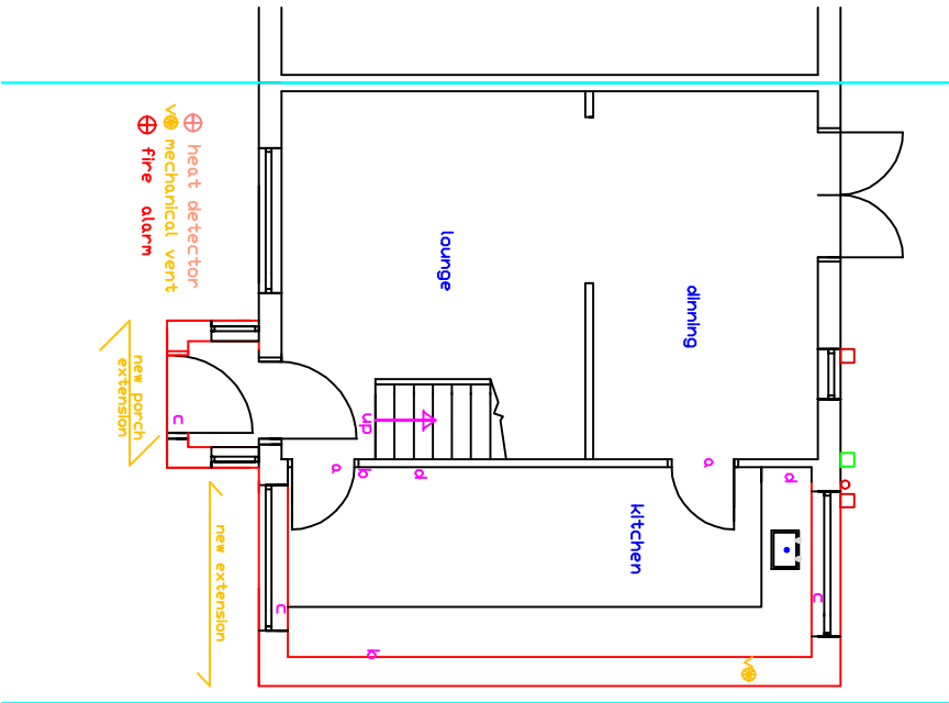
PROPOSED GROUND FLOOR 1:100
