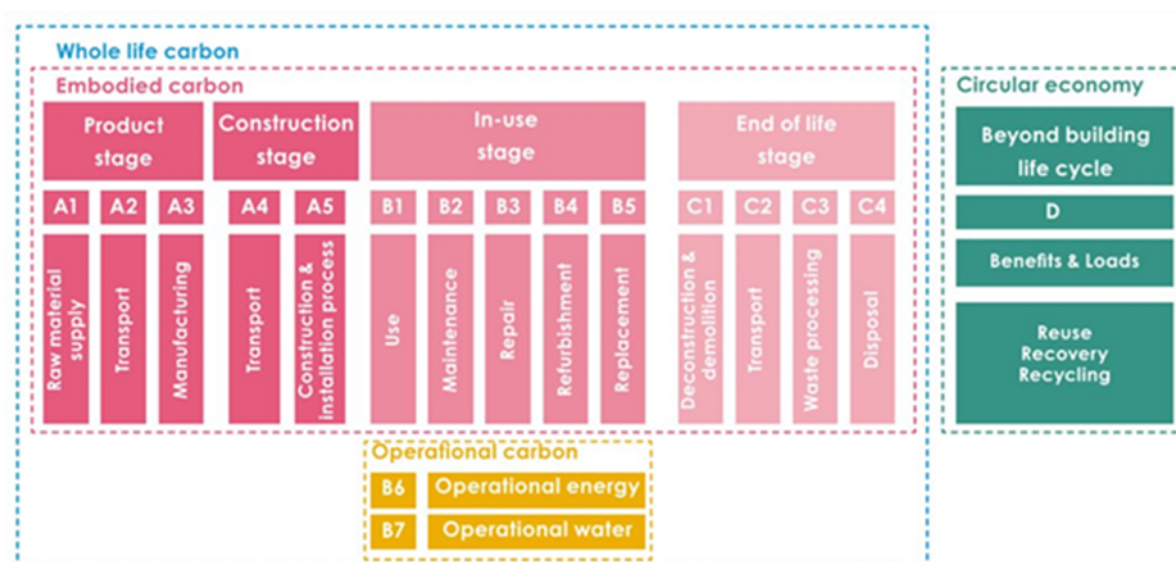
Figure 3 - Diagram showing the stages of a lifecycle GHG emissions assessment, taken from the LETI Embodied Carbon Primer (2020) Diagram based on lifecycle stages set out in BS EN 15978
