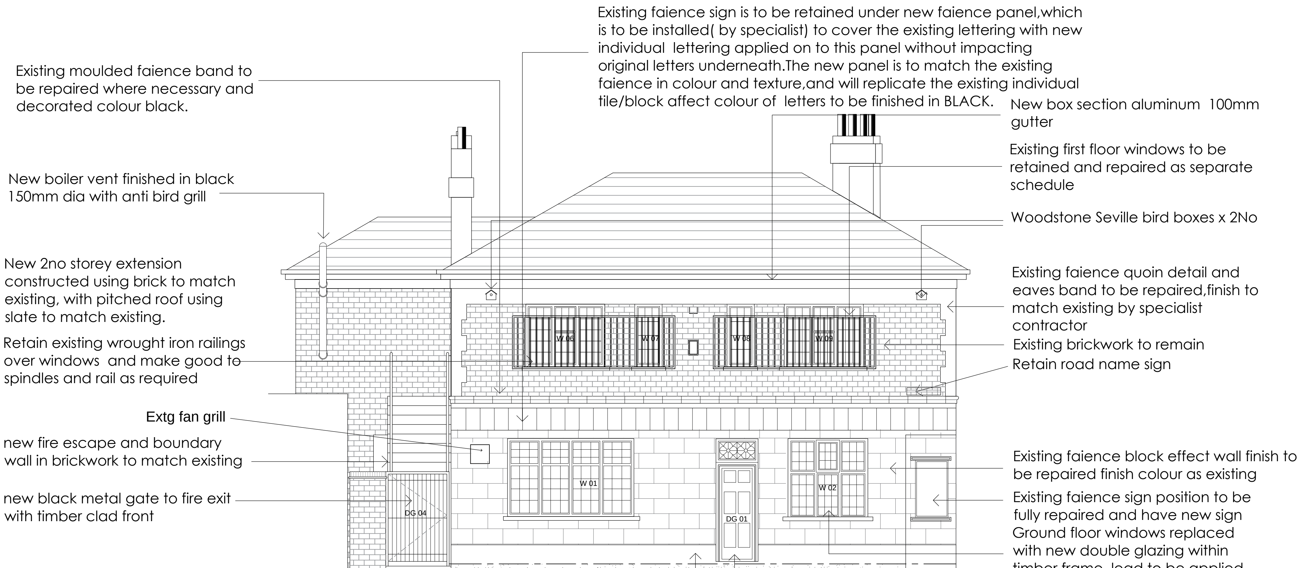
ELEVATION A - SILK STREET Scale 1:50 @ A1 Existing faience block plinth finish to be repaired and decorated colour black
