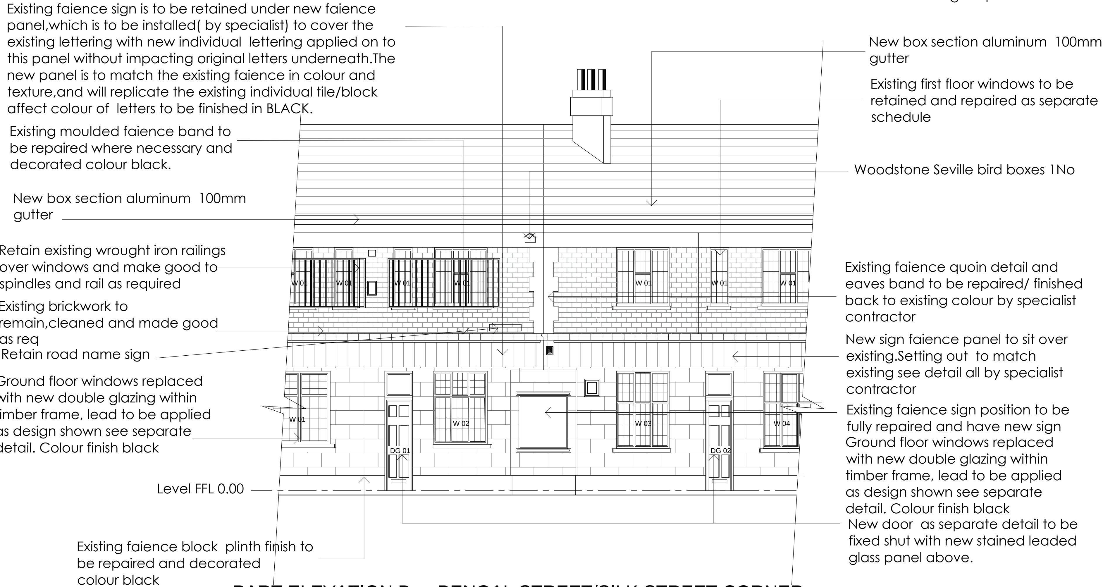
PART ELEVATION B - BENGAL STREET/SILK STREET CORNER Scale 1:50 @ A1
