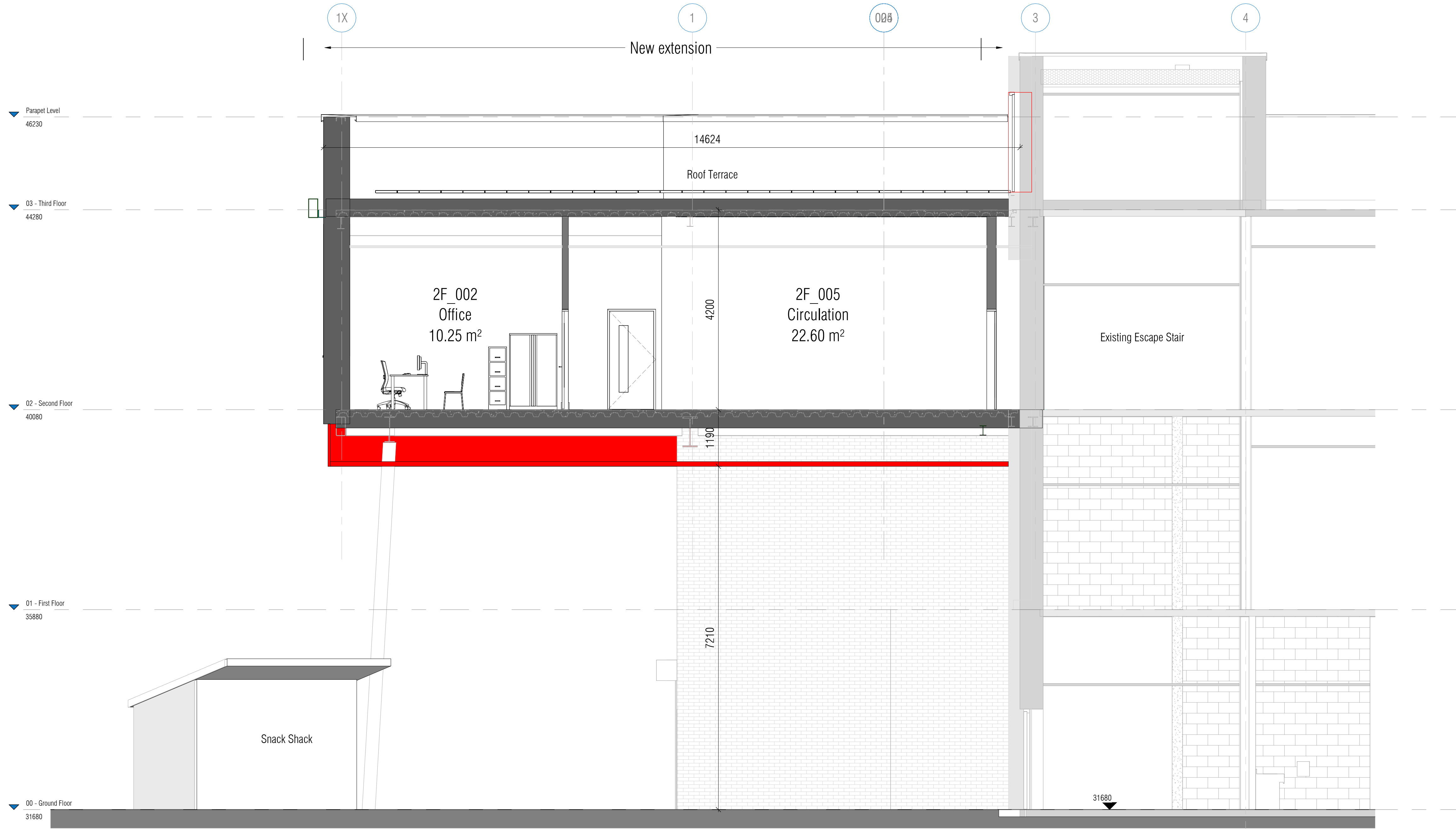
E Section E-E Planning 1 : 50
