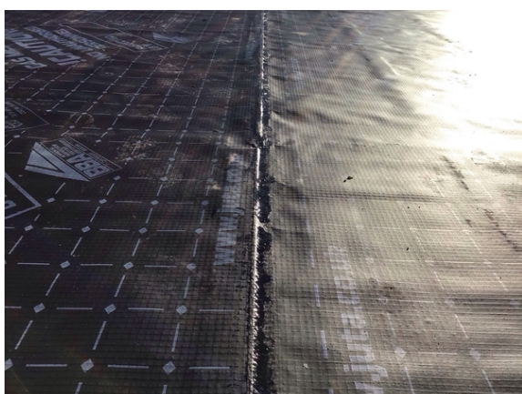
Hand welded membrane lap joint
