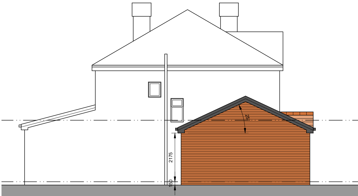
East Facing Side Elevation
