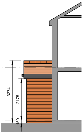
West Facing Side Elevation
