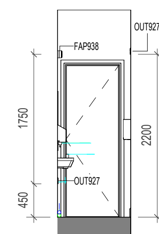
[12] ELEVATION 12 1:50
