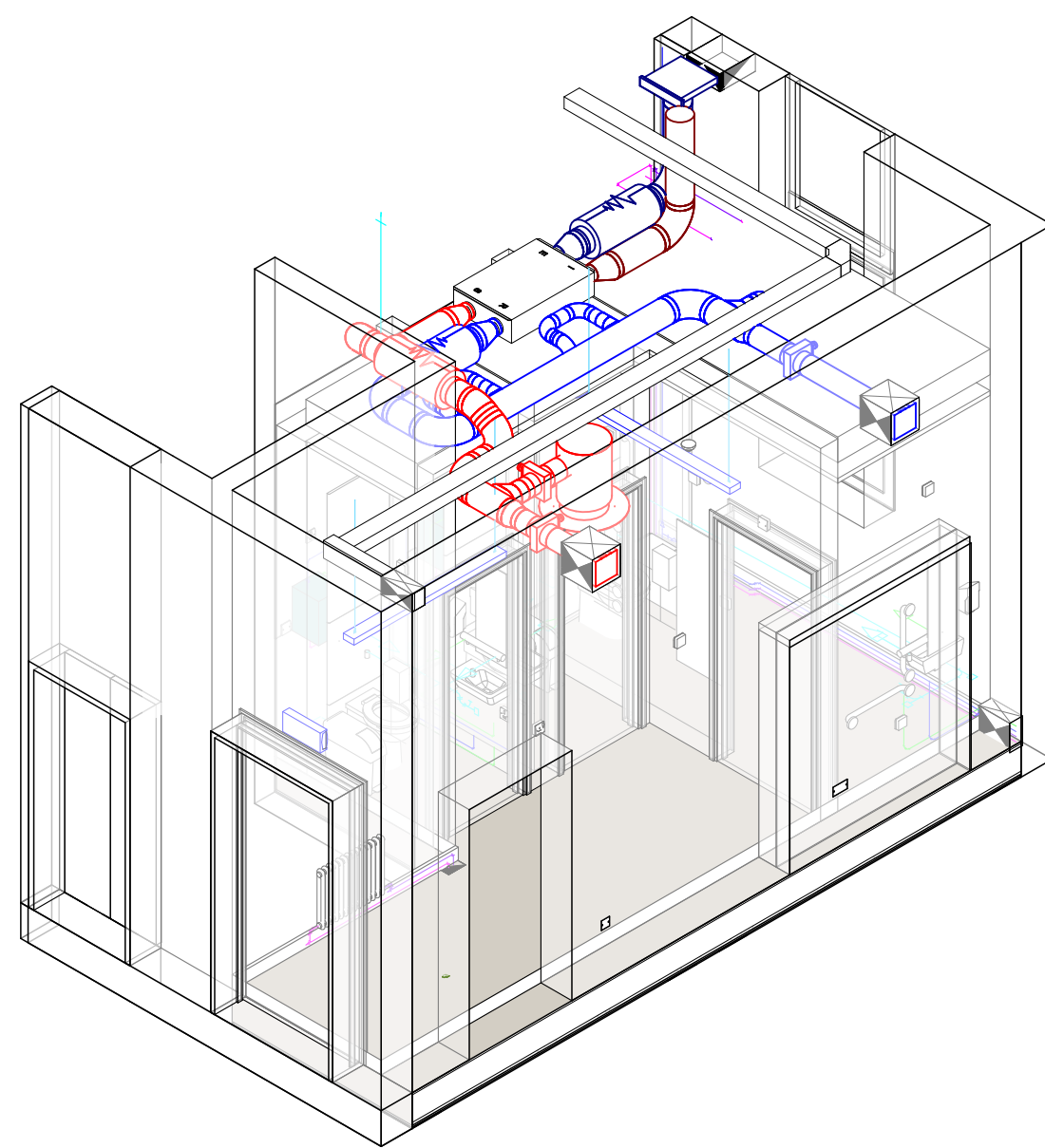
14 1.056 WCs Isometric View
