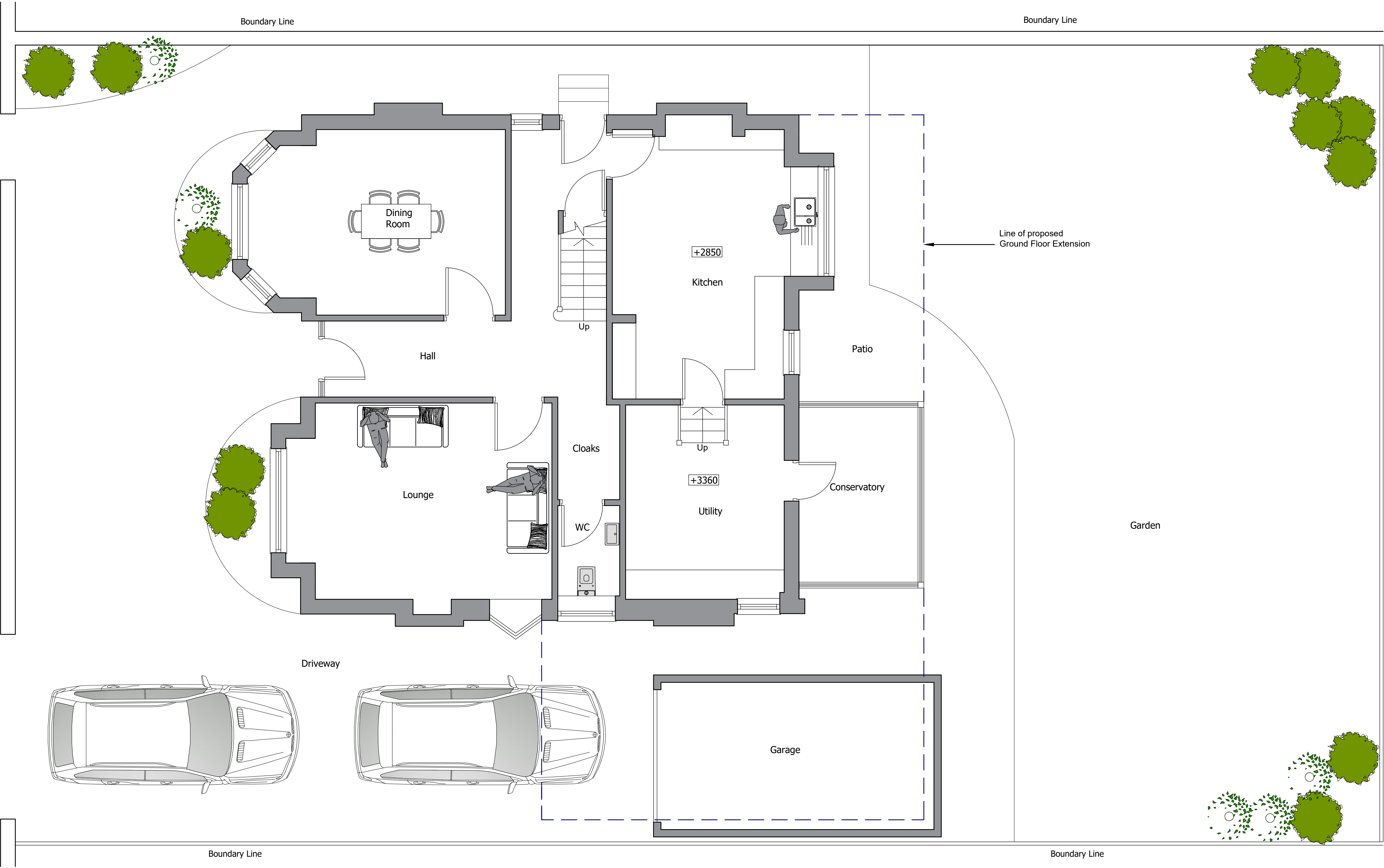
Ground Floor
