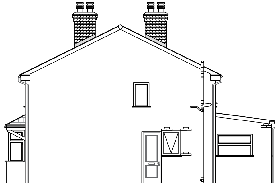
Side Existing Elevation Viewed from 234 Brantingham Road
