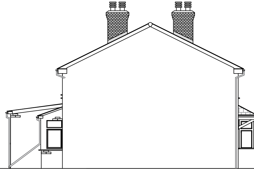
Side Existing Elevation Viewed from 238 Brantingham Road
