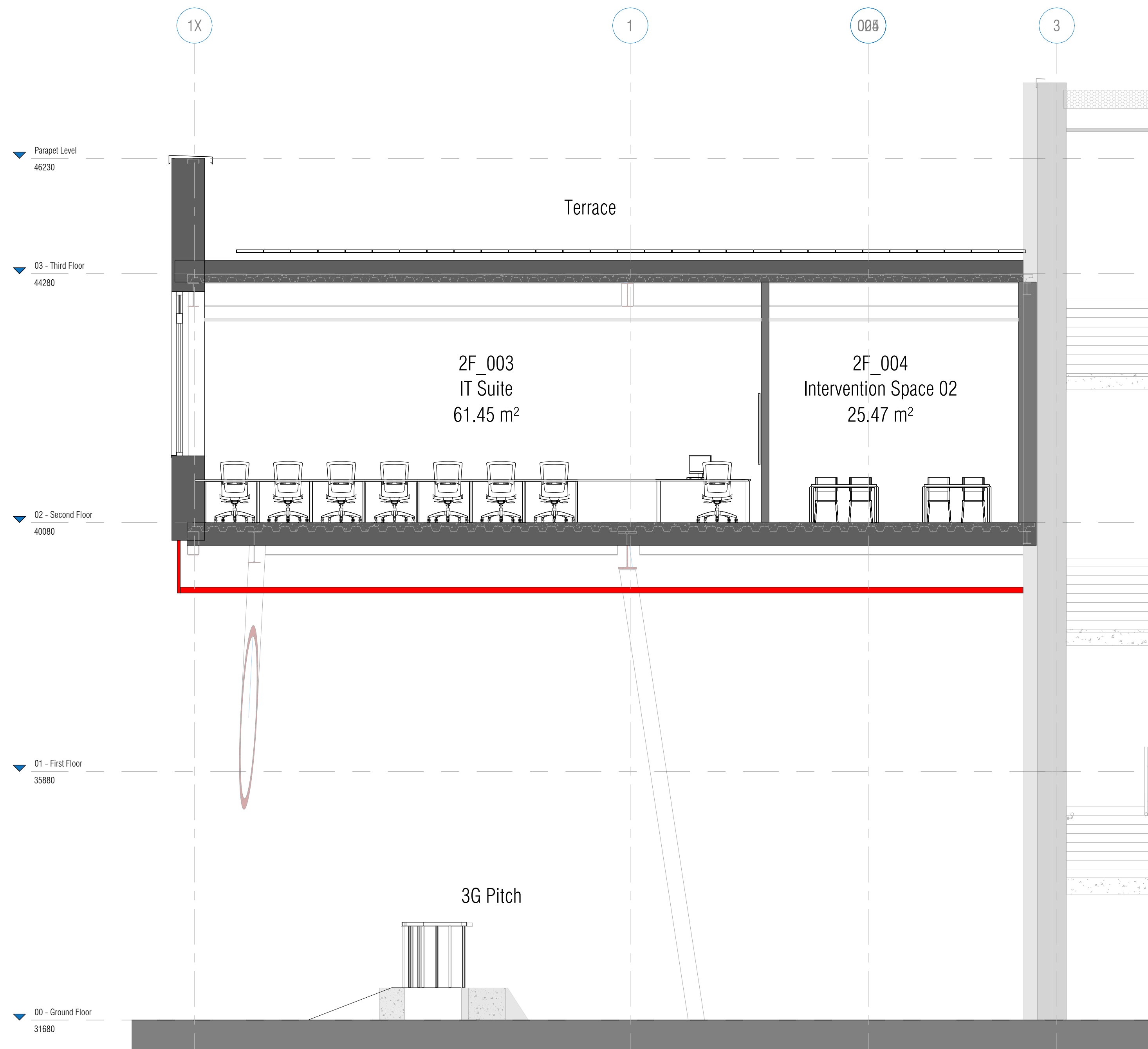
C Section C-C Planning 1 : 50
