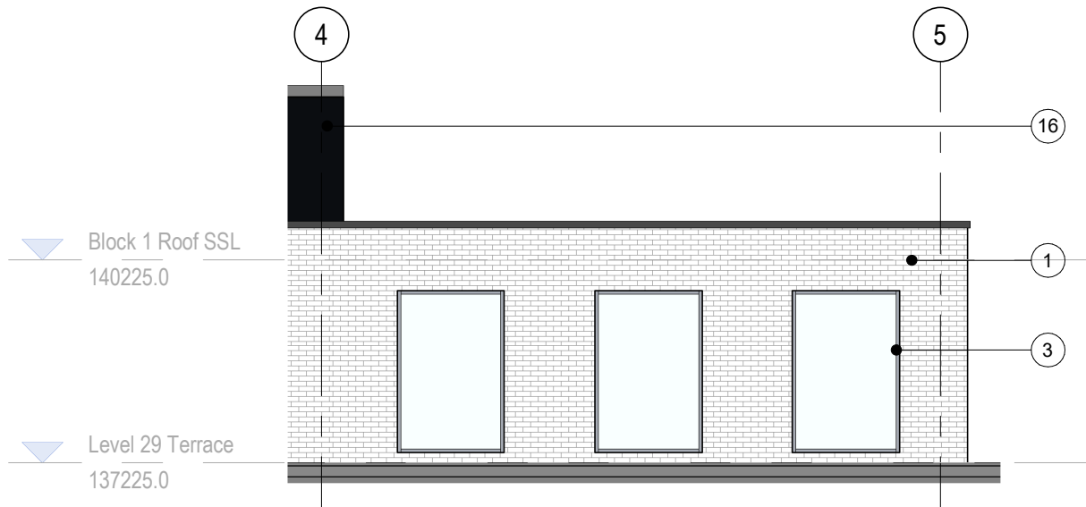
Block 1 - Level 29 Amenity Glazing - Elevation B 1 : 100
