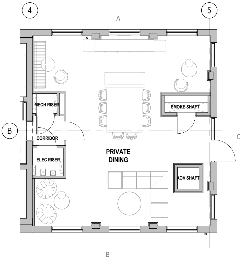
Block 1 - Level 29 Amenity Glazing 1 : 100
