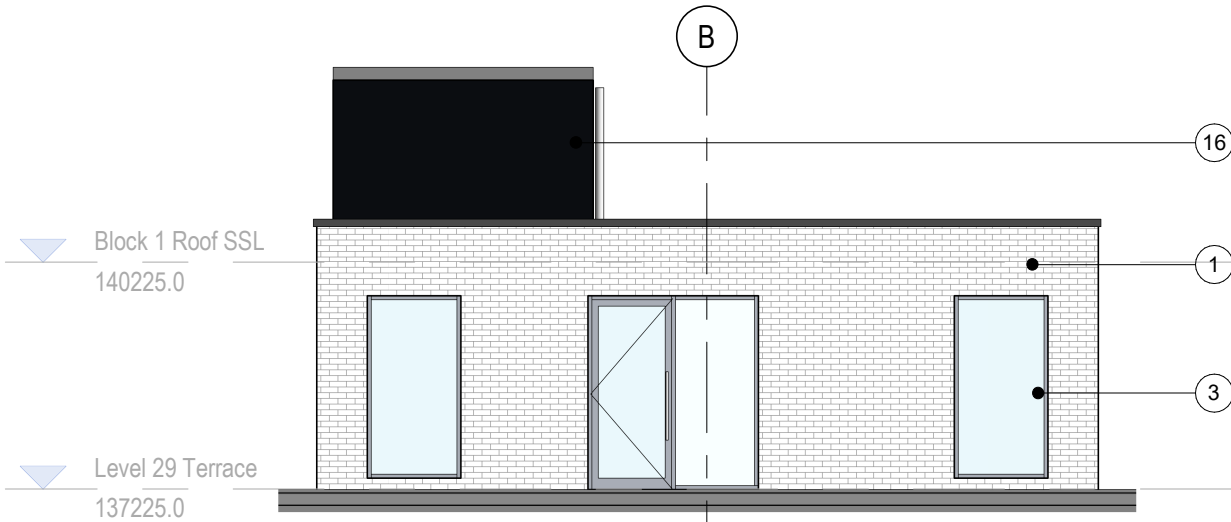
Block 1 - Level 29 Amenity Glazing - Elevation C 1 : 100
