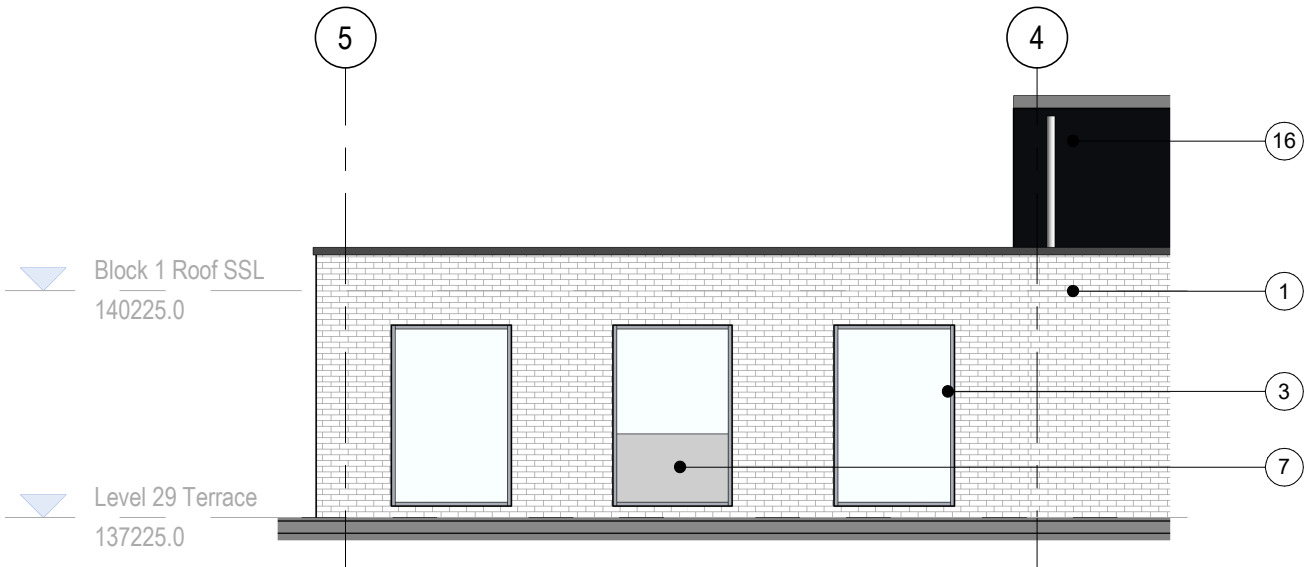
Block 1 - Level 29 Amenity Glazing - Elevation A 1 : 100
