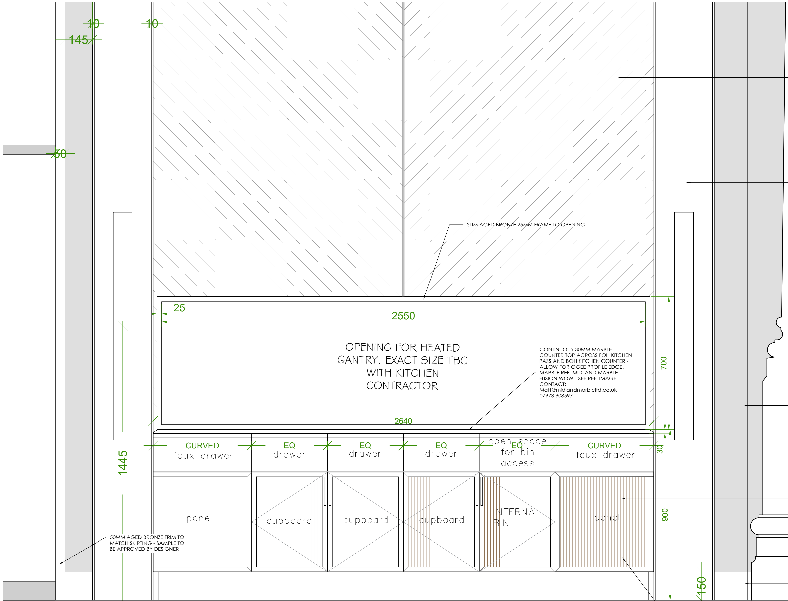
KITCHEN PASS ELEVATION A-A SCALE: 1:10 @ A1
