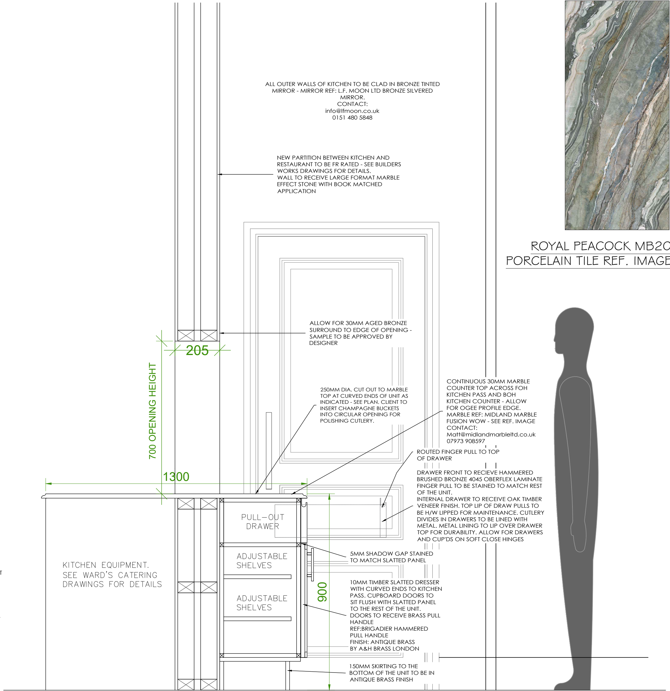
KITCHEN PASS SECTION THROUGH B-B SCALE: 1:10 @ A1
