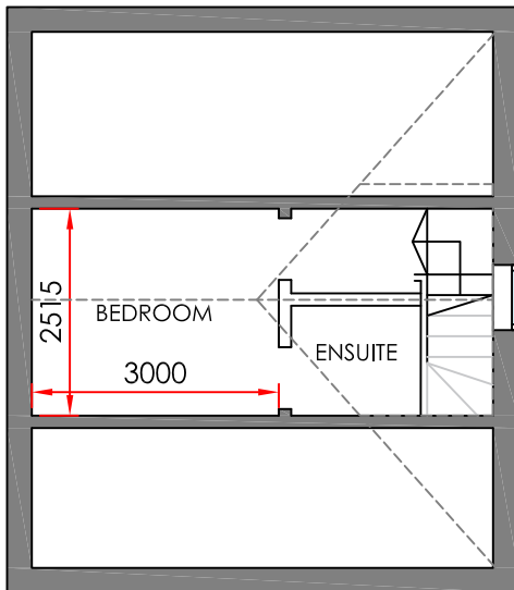
PROPOSED LOFT FLOOR PLAN
