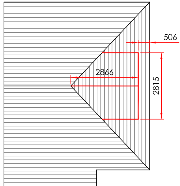
PROPOSED ROOF FLOOR PLAN
