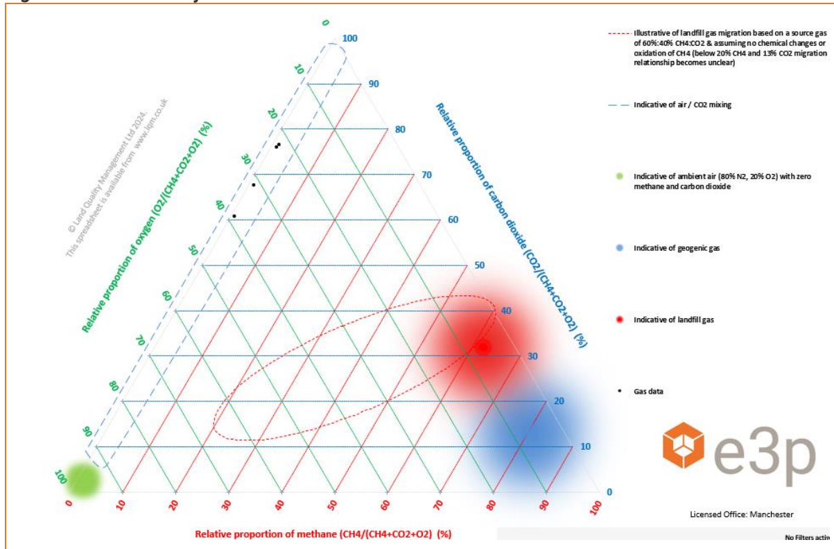
Figure 4 Ternary Plot
