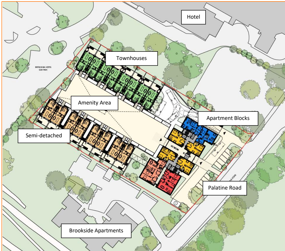
Figure 4: Proposed Site Layout
