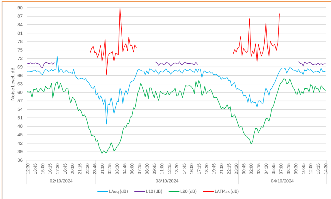
Figure 6: LT1 Façade Monitoring Results
