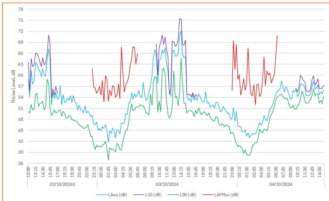
Figure 7: LT2 Façade Monitoring Results
