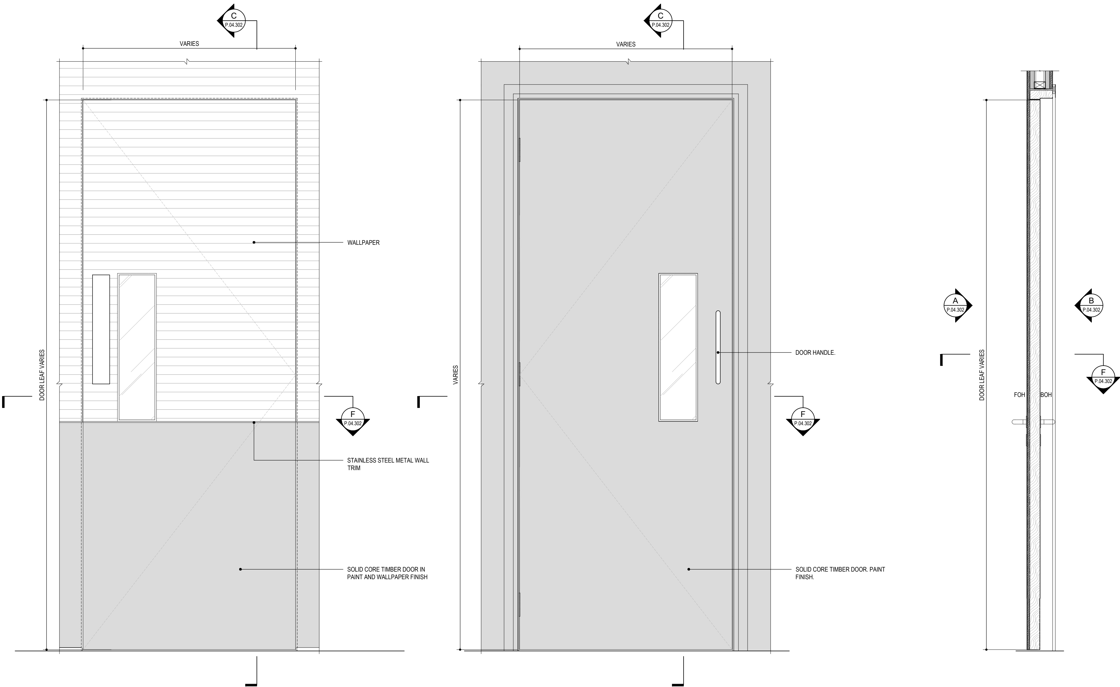
A DOOR TYPE T01 - ELEVATION SCALE: 1:10@A1; 1:20@A3
