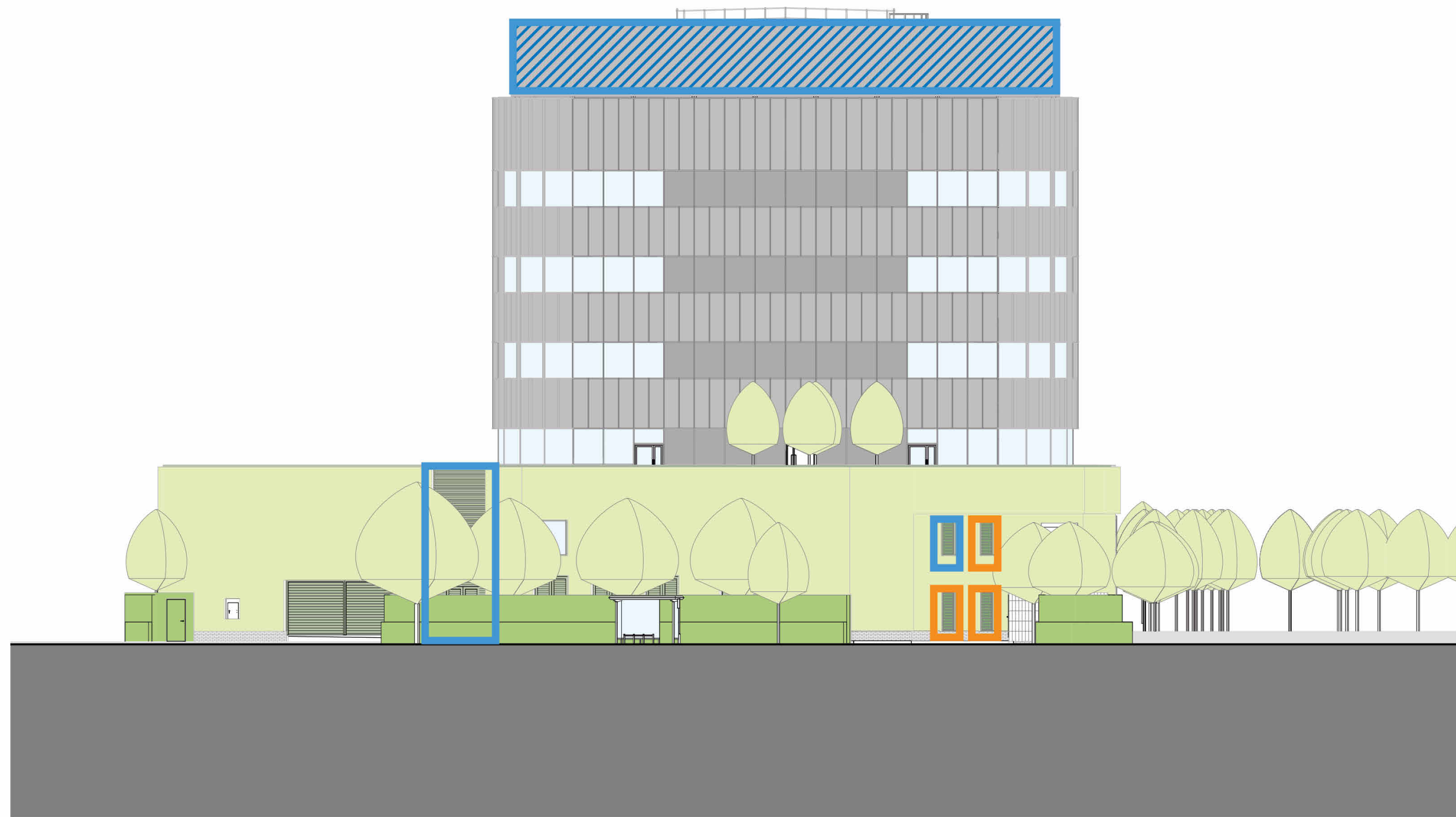
West Elevation
