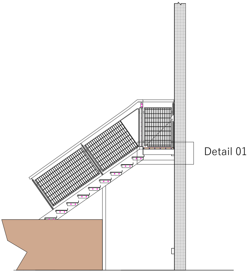
Section A-A (Existing Staircase 01)
