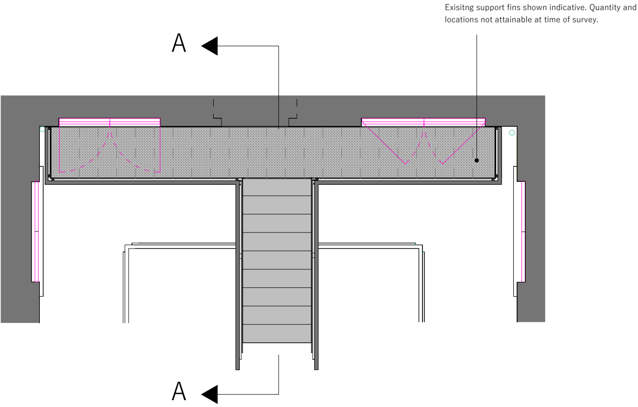
Proposed Courtyard Plan Section c/w Staircase 02
