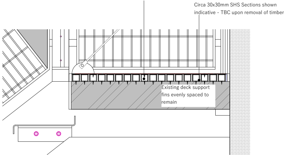
Detail 01 - Proposed
