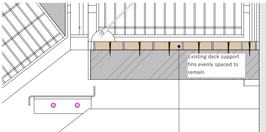
Detail 01 - Existing
