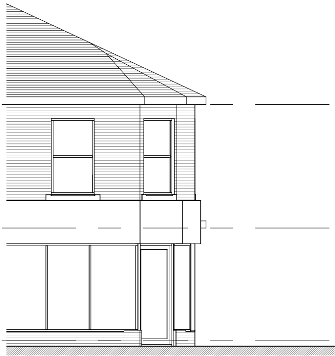
1 Front - Proposed 1 : 100
