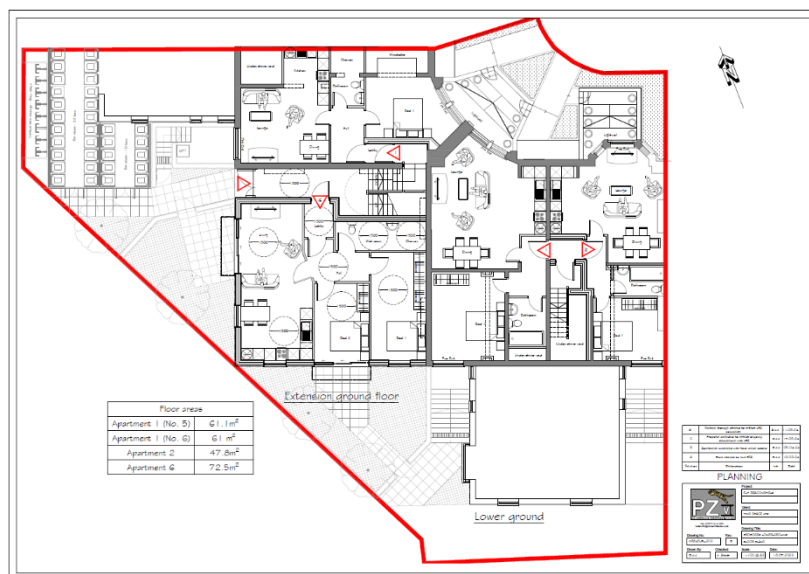
Figure 14. Ground floor plan
