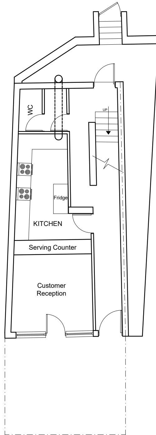
PRE EXISTING GROUND FLOOR PLAN
