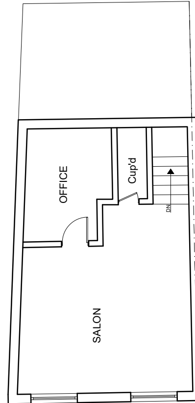
PRE EXISTING FIRST FLOOR PLAN
