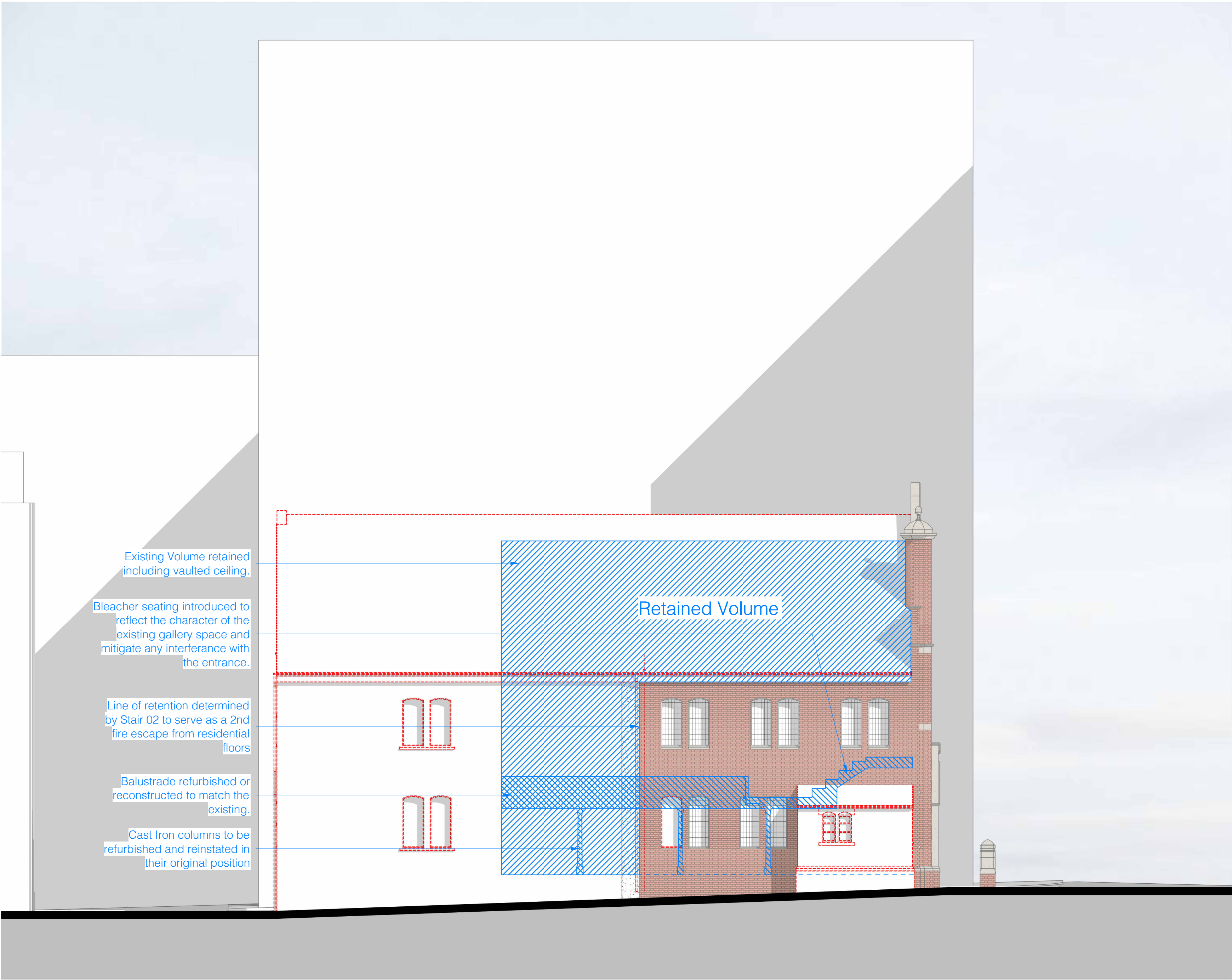
1 Elevation - SW Demolition 1 : 100
