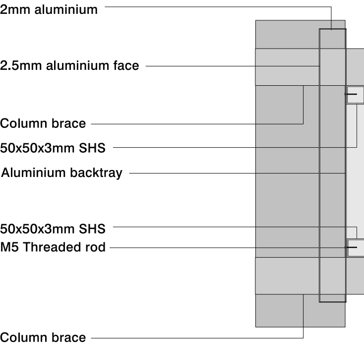
Section Through - Scale 1:10
