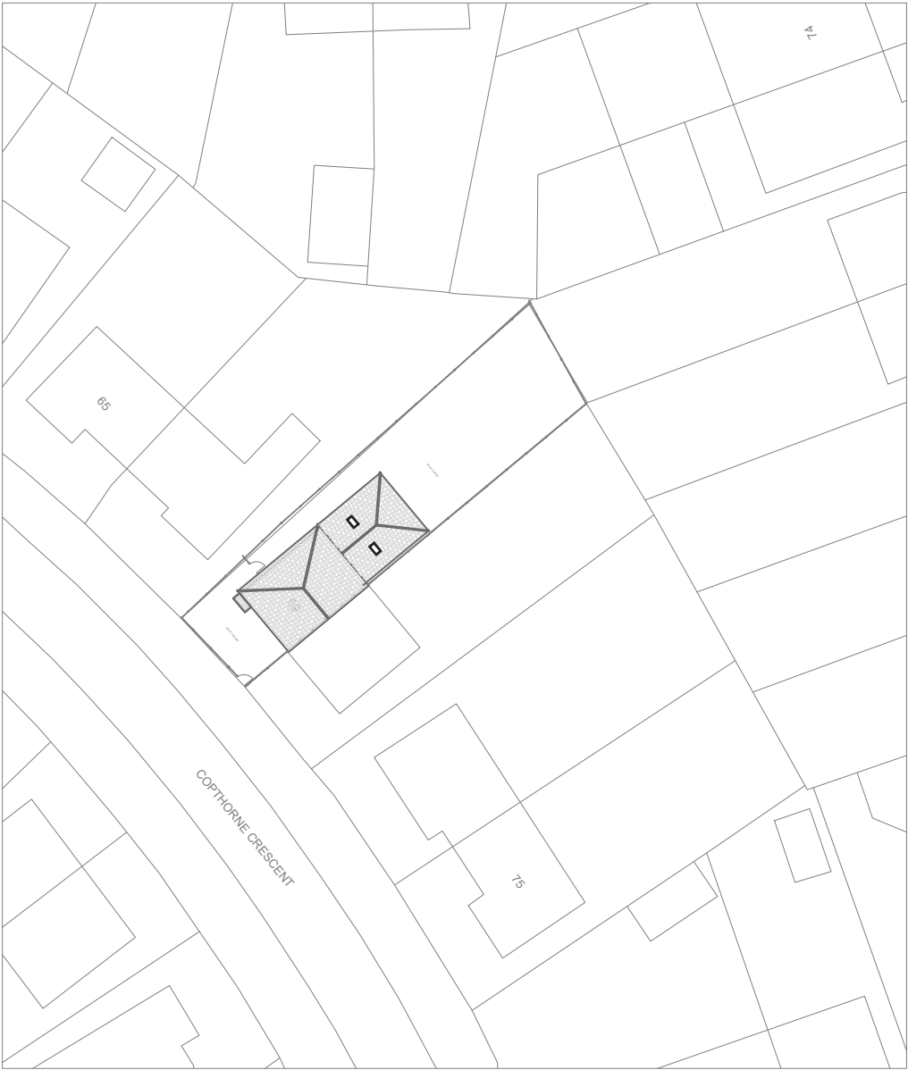
PROPOSED SITE/BLOCK PLAN @ Scale: 1: 500
