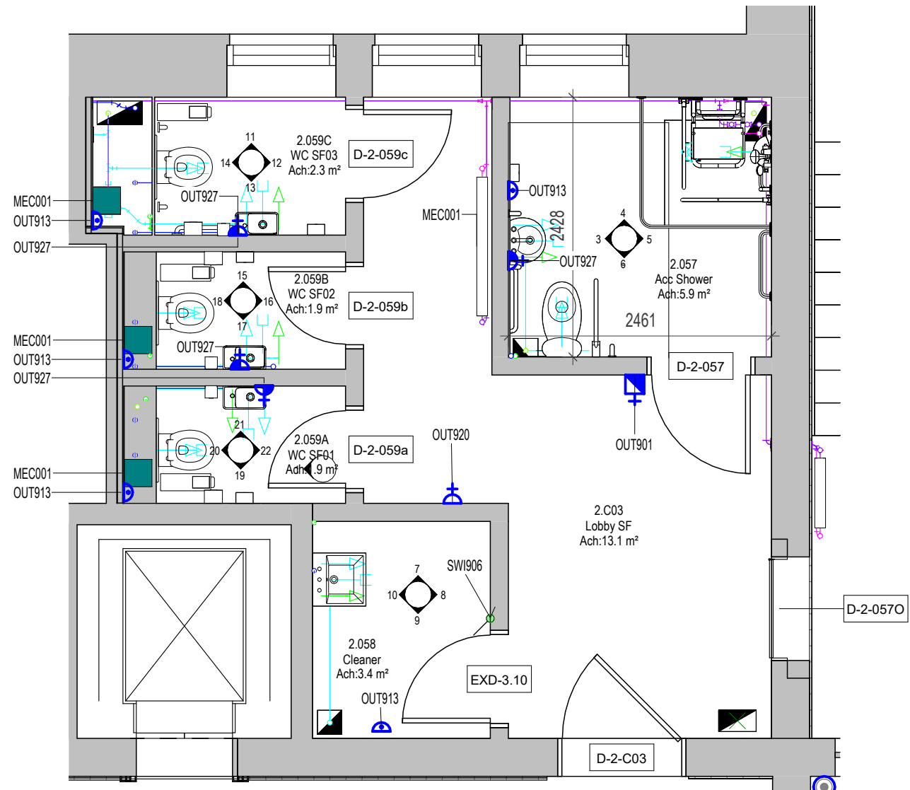
1 2.057,058,059 - WC Block 1 : 50
