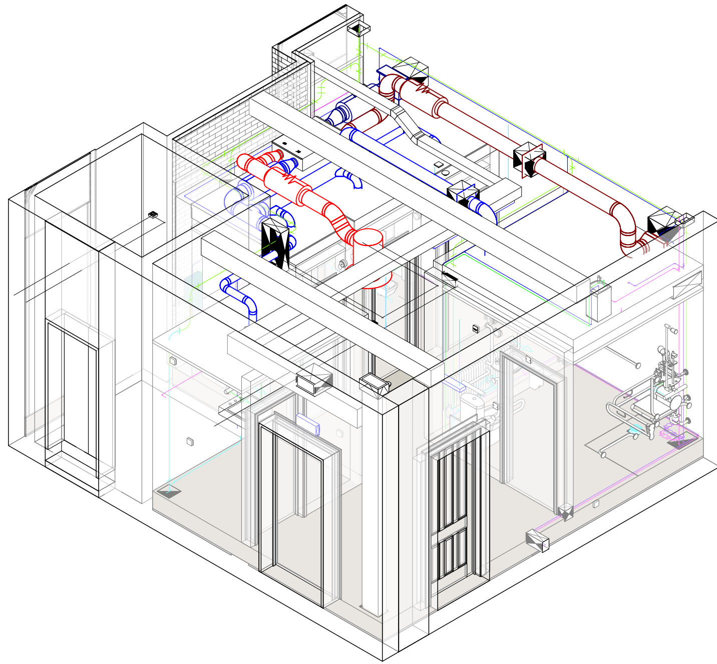
2 2.057,058,059 - WC Block Isometric View
