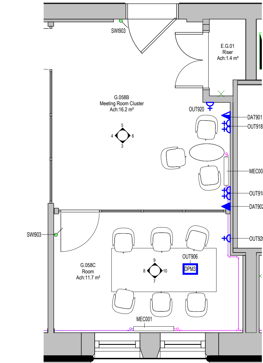
1 Meeting Room G.058B and G.058C Floor Plan 1 : 50
