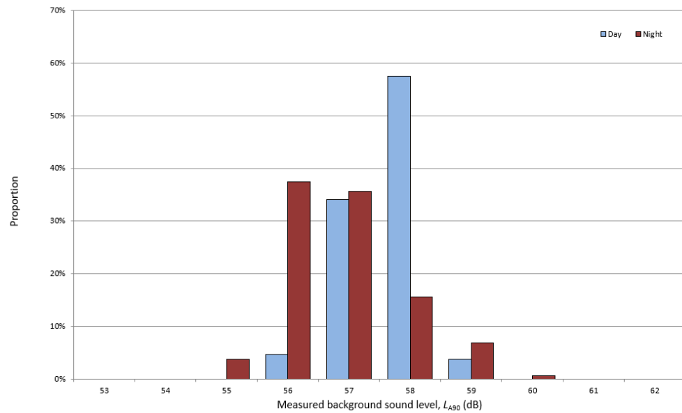
Figure 4 Measured background sound levels – Histogram
