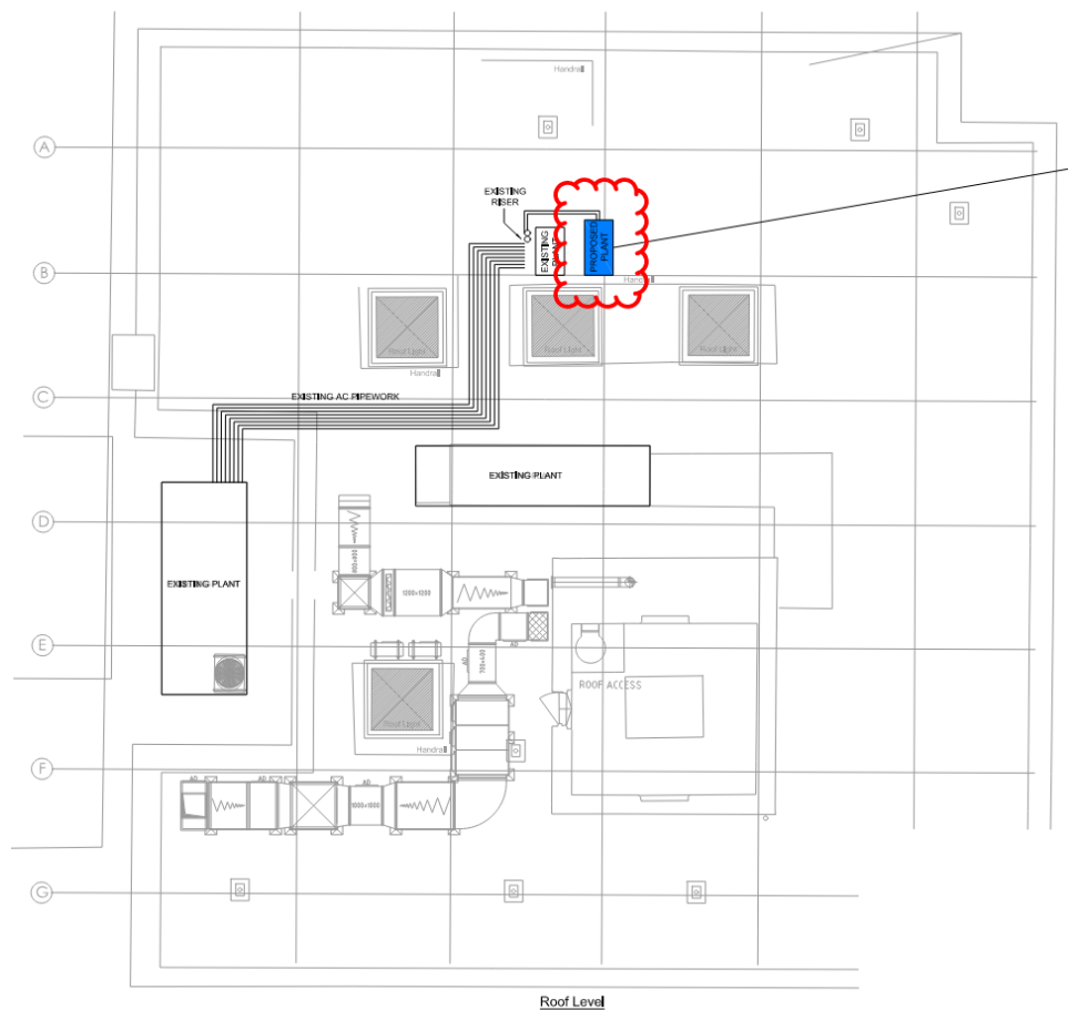
Figure 2 Proposed condenser unit location
