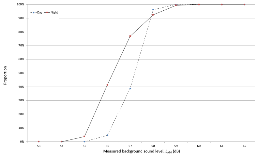
Figure 5 Measured background sound levels – Cumulative
