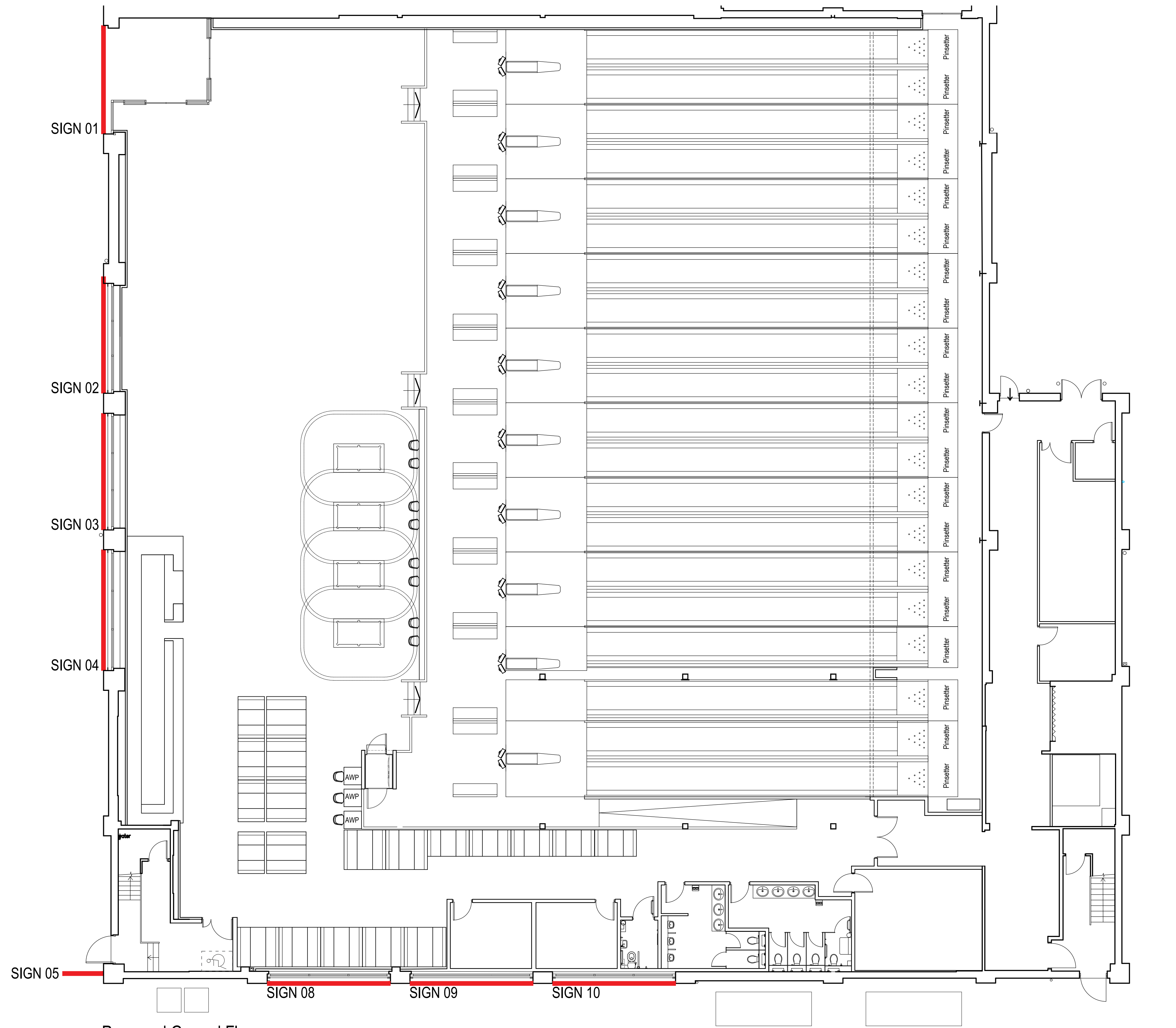
Proposed Ground Floor Scale 1:100@A0 Subject to LA Approval
