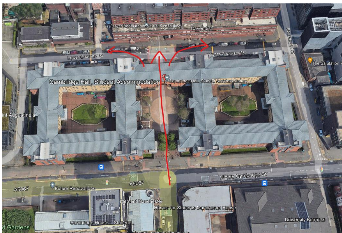
Figure 8.4: Aerial view of the existing site and existing surroundings, with sketches showing the locations and directions of expected accelerated winds.
