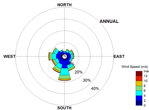
Figure 8.1 Annual wind rose obtained from the wind data recorded at Manchester Airport (10m height) during the years 1991 to 2015.
