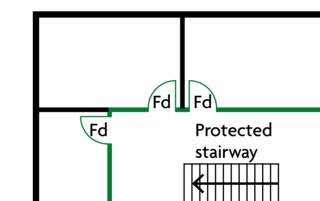
a. Ground Floor Layout
