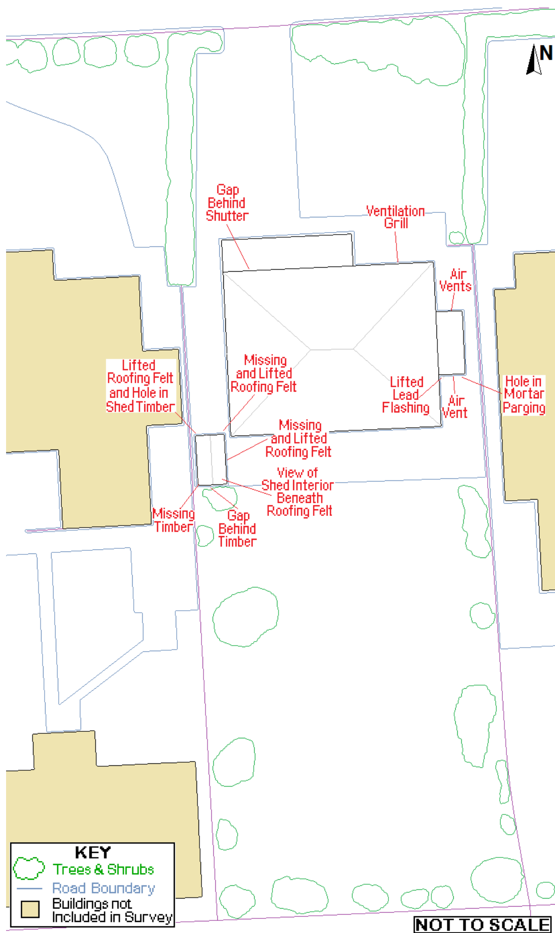
Fig 5 – Plan Showing Results of Preliminary Daylight Evidence and Opportunity Survey and Assessment.
