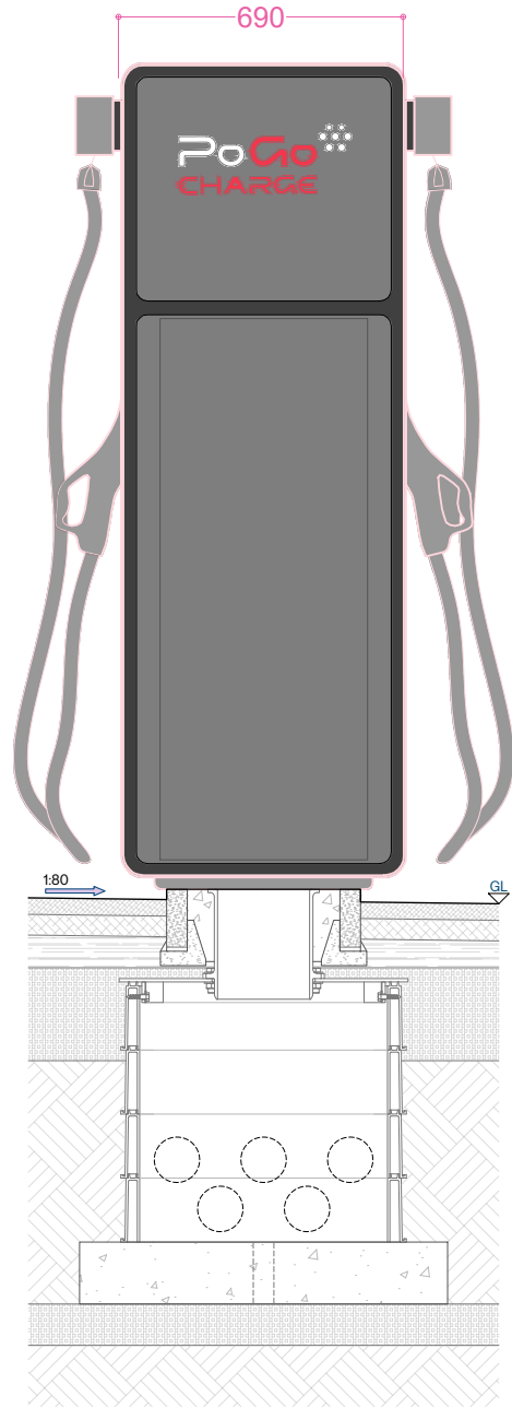
Rear Sectional Elevation
