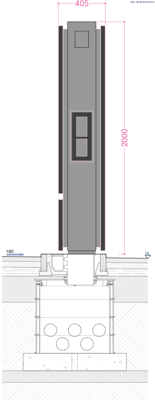
Side Sectional Elevation
