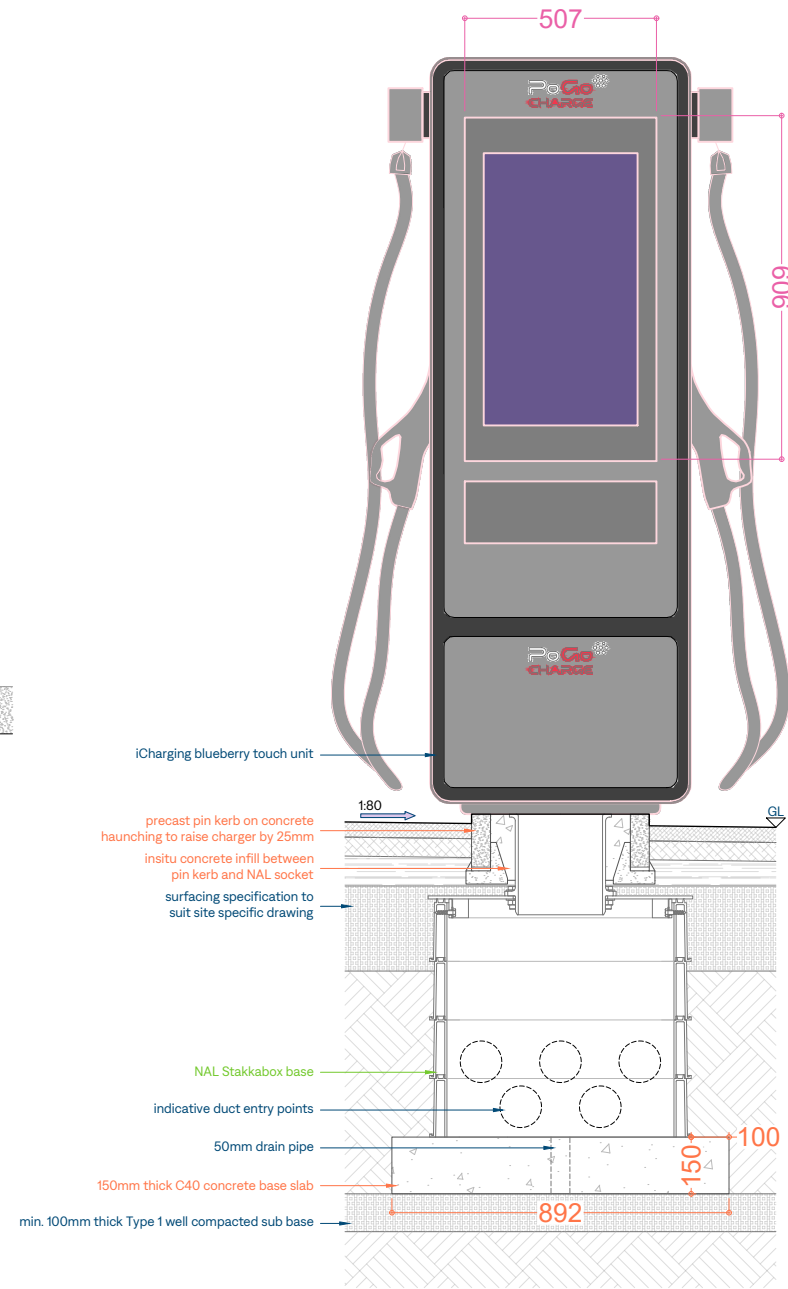
Front Sectional Elevation
