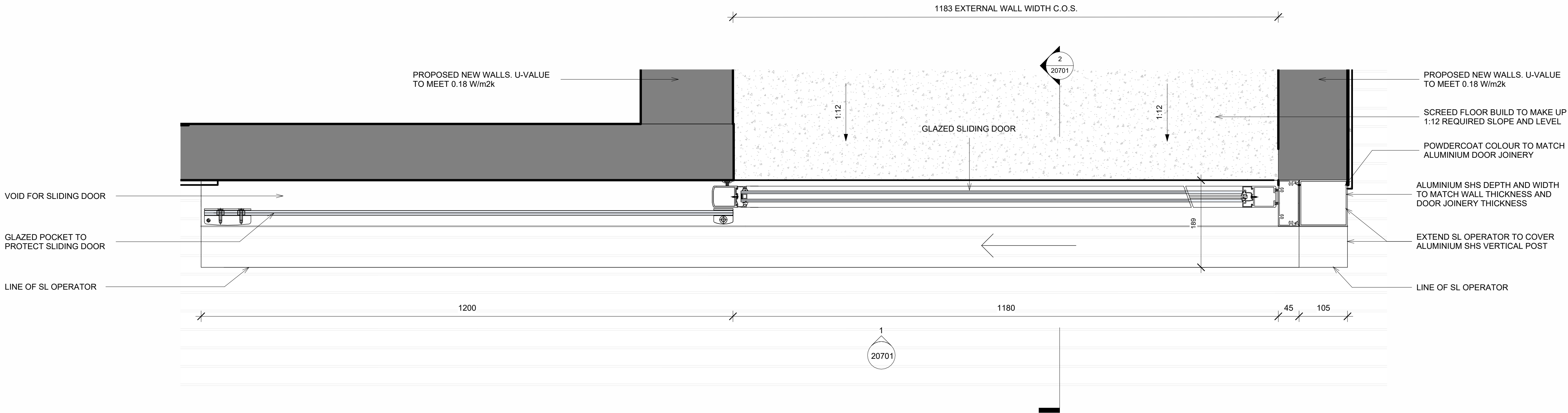
PROPOSED EOJ ENTRANCE DOOR PLAN 1 : 5
