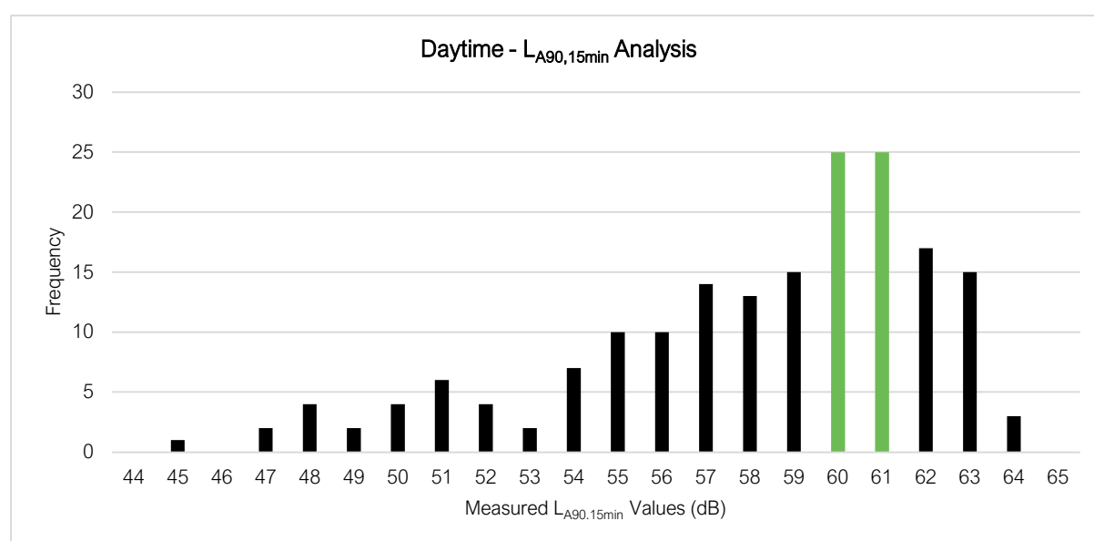
Figure 3 – Background Sound Level Analysis (During Proposed Operational Hours)
