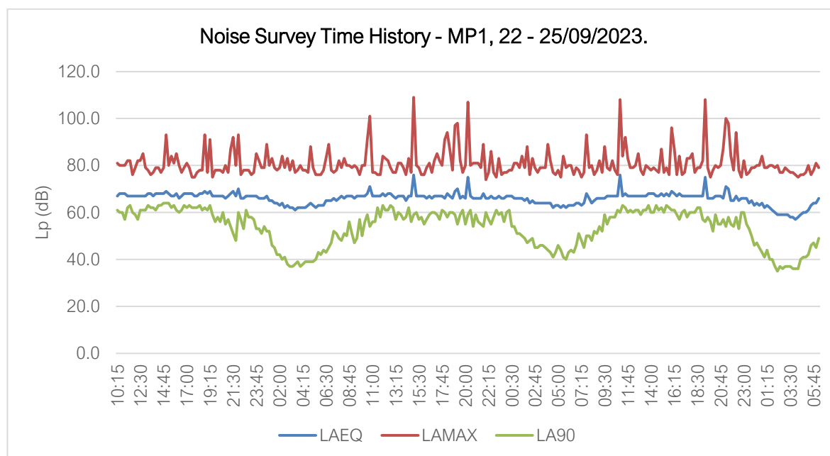
Figure 5 – MP1 Noise Survey Time History
