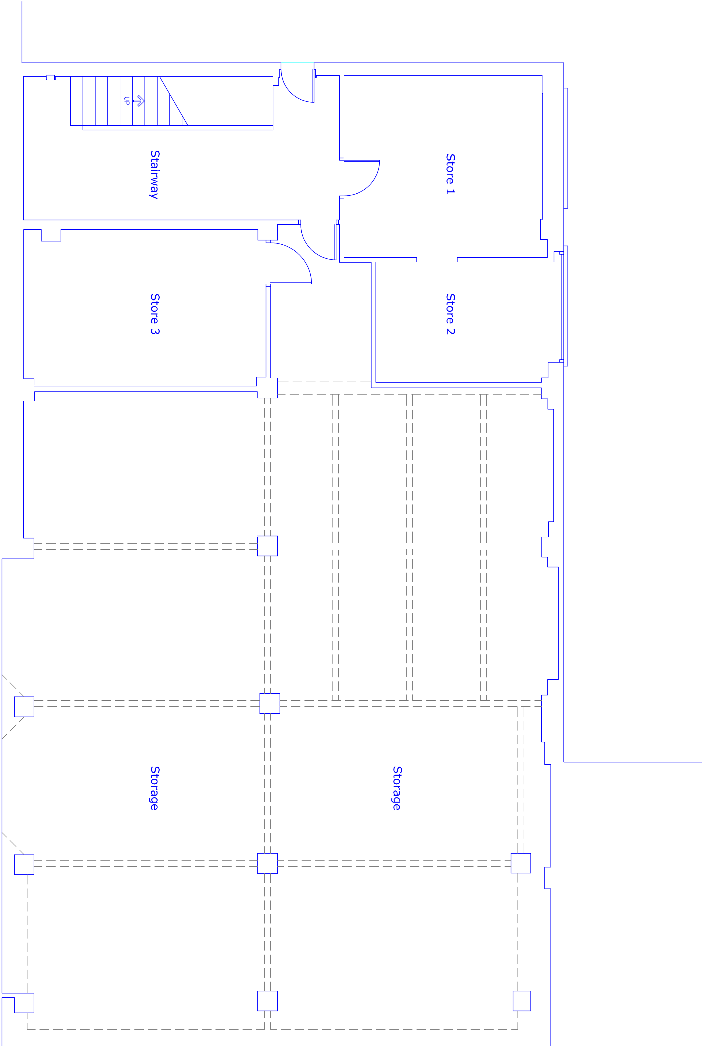
Existing Basement Floor Plan
