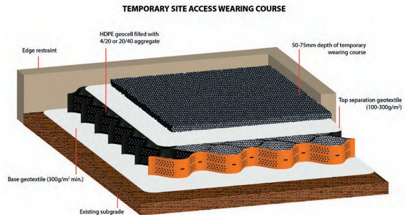
Figure 5: A geocell surface used during construction needs to be protected by a temporary wearing course and an upper geotextile is required to prevent mud from migrating down into the infill [image courtesy of Core LP].
