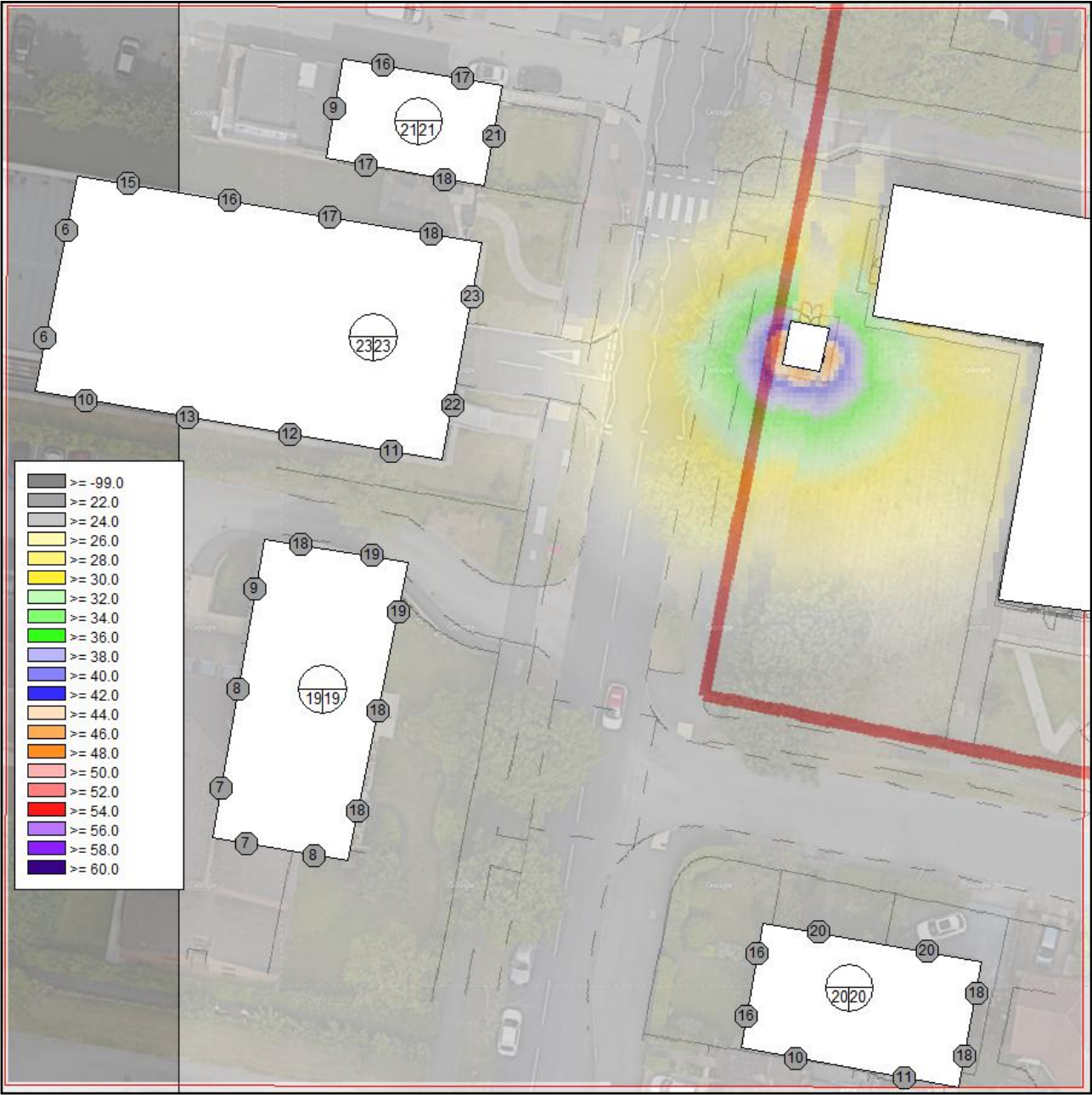
Figure 5.1: Calculated Sound Level (dBA) Based on Measured Data with Substation Operational
