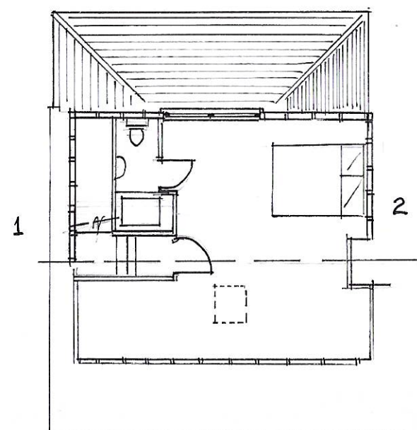
2ND FLOOR
