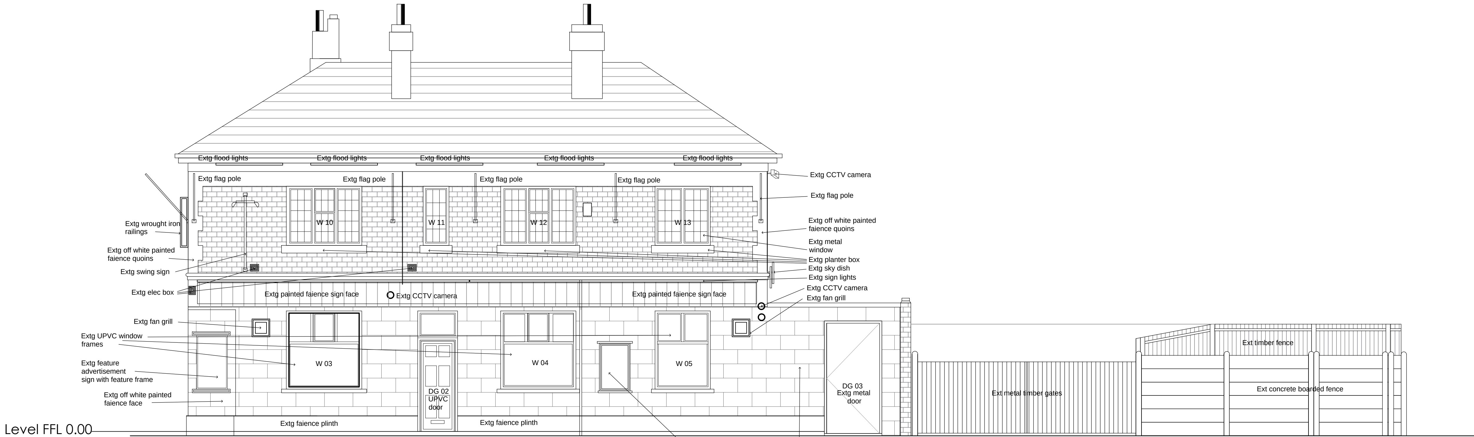
ELEVATION C - BENGAL STREET Scale 1:50 @ A1
