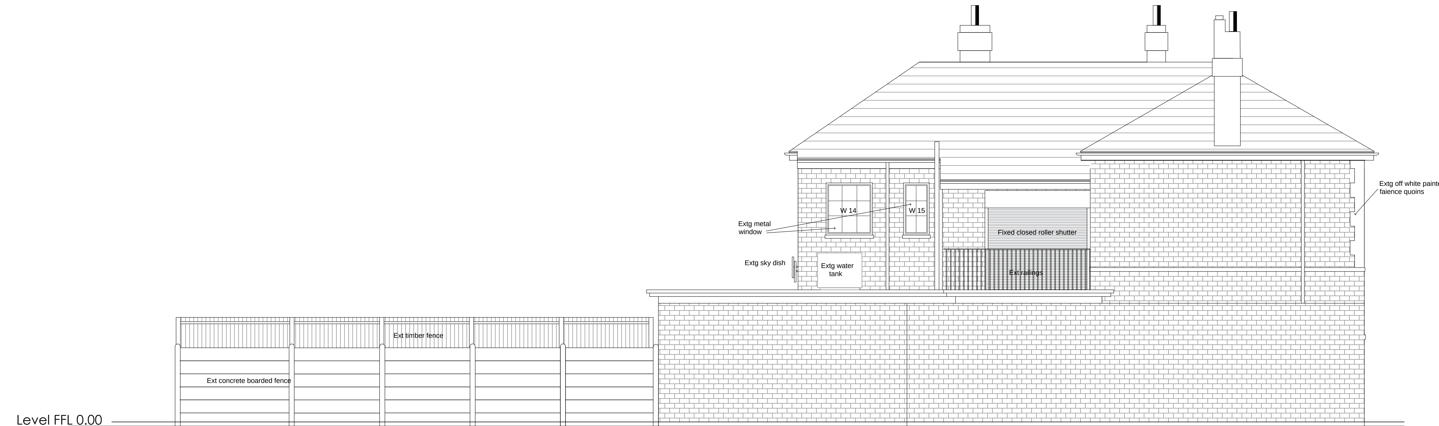
ELEVATION D - FROM SUB STATION Scale 1:50 @ A1
