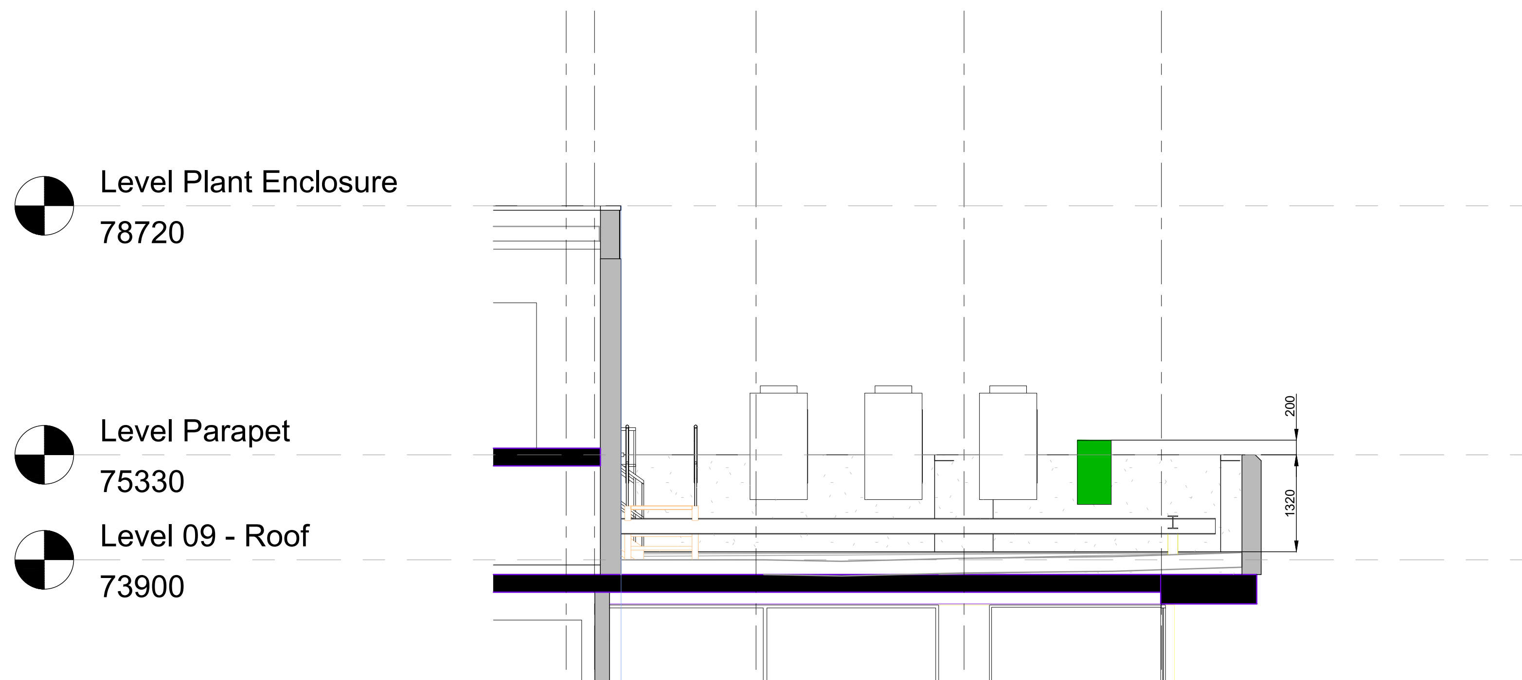
SECTION - AYTOUN STREET
