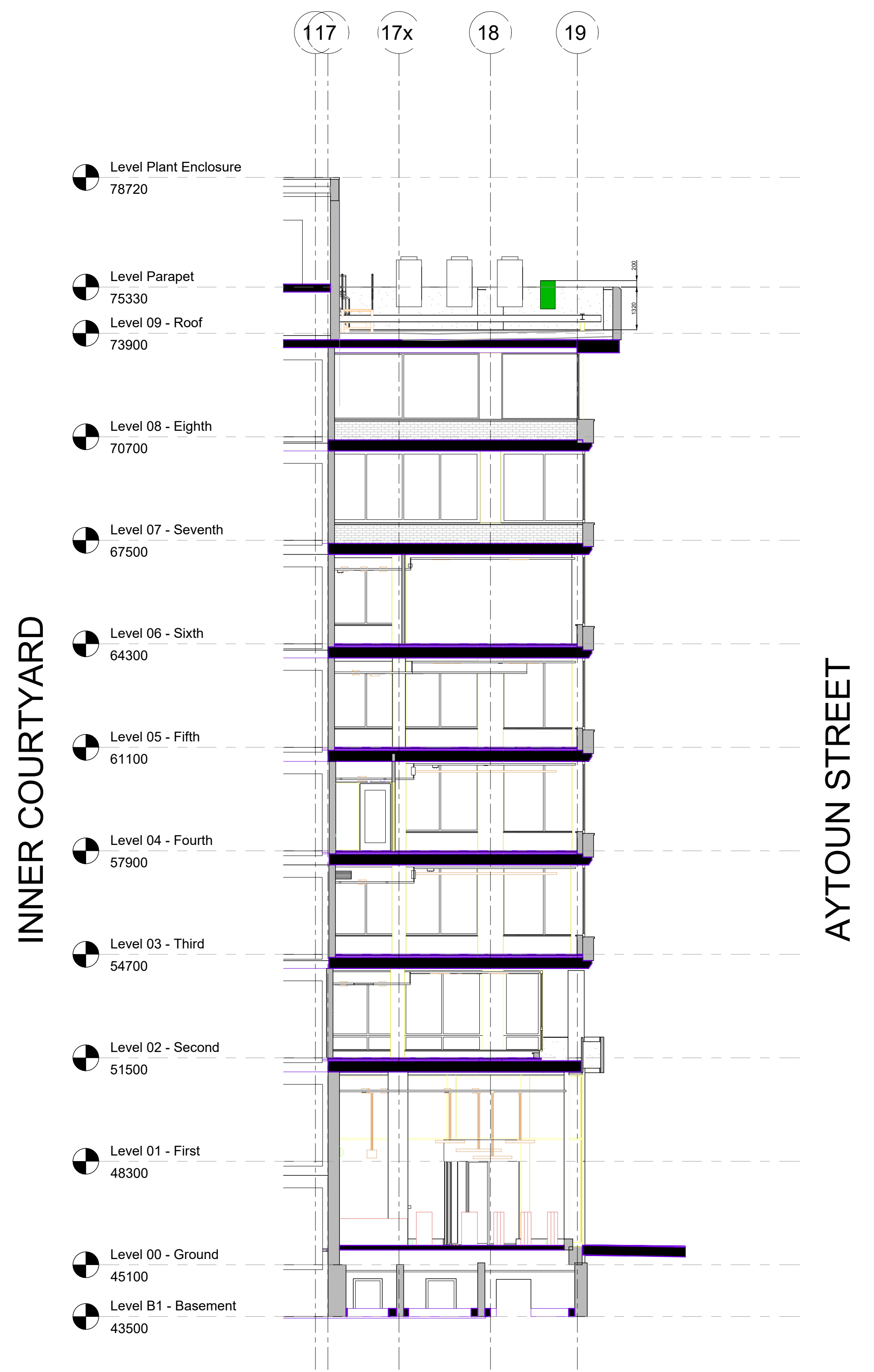
SECTION - AYTOUN STREET
