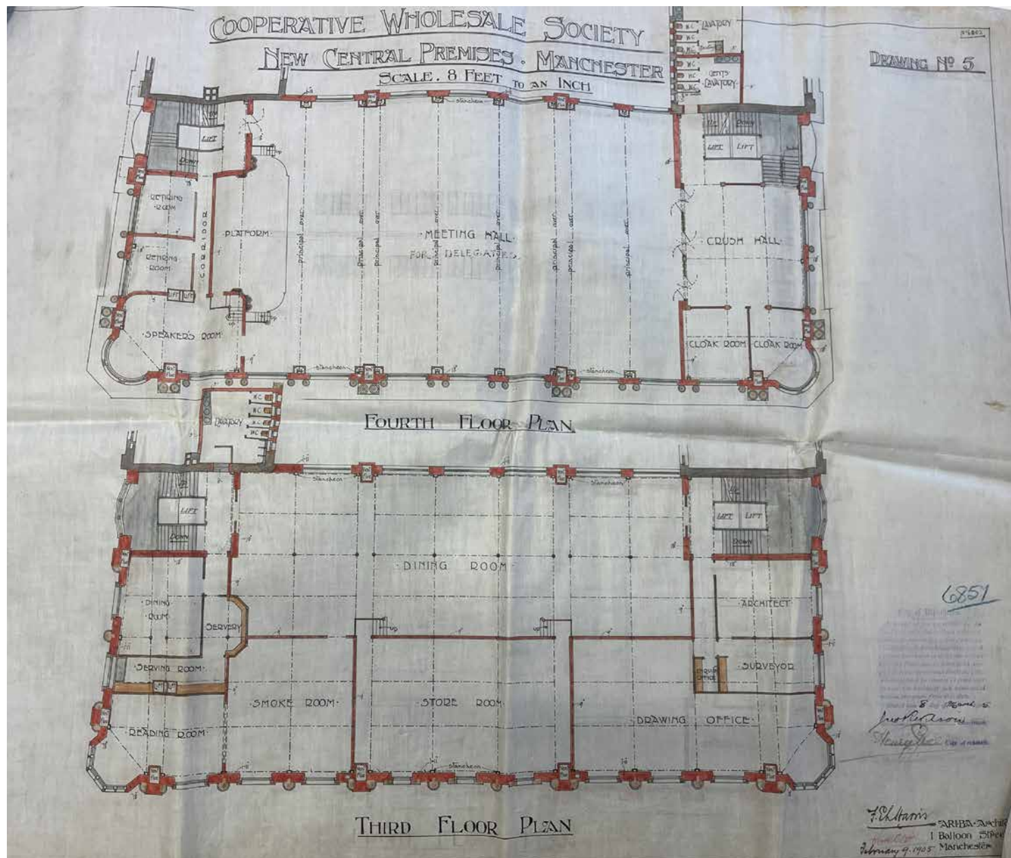
2.21 1905 proposed Hanover House third and fourth-floor plans (Manchester Archives)
