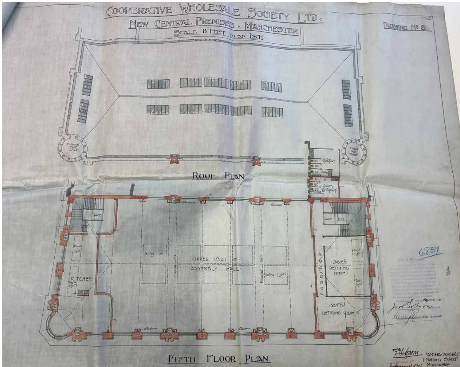
2.22 1905 proposed fifth-floor and roof plans of Hanover House (Manchester Archives)
