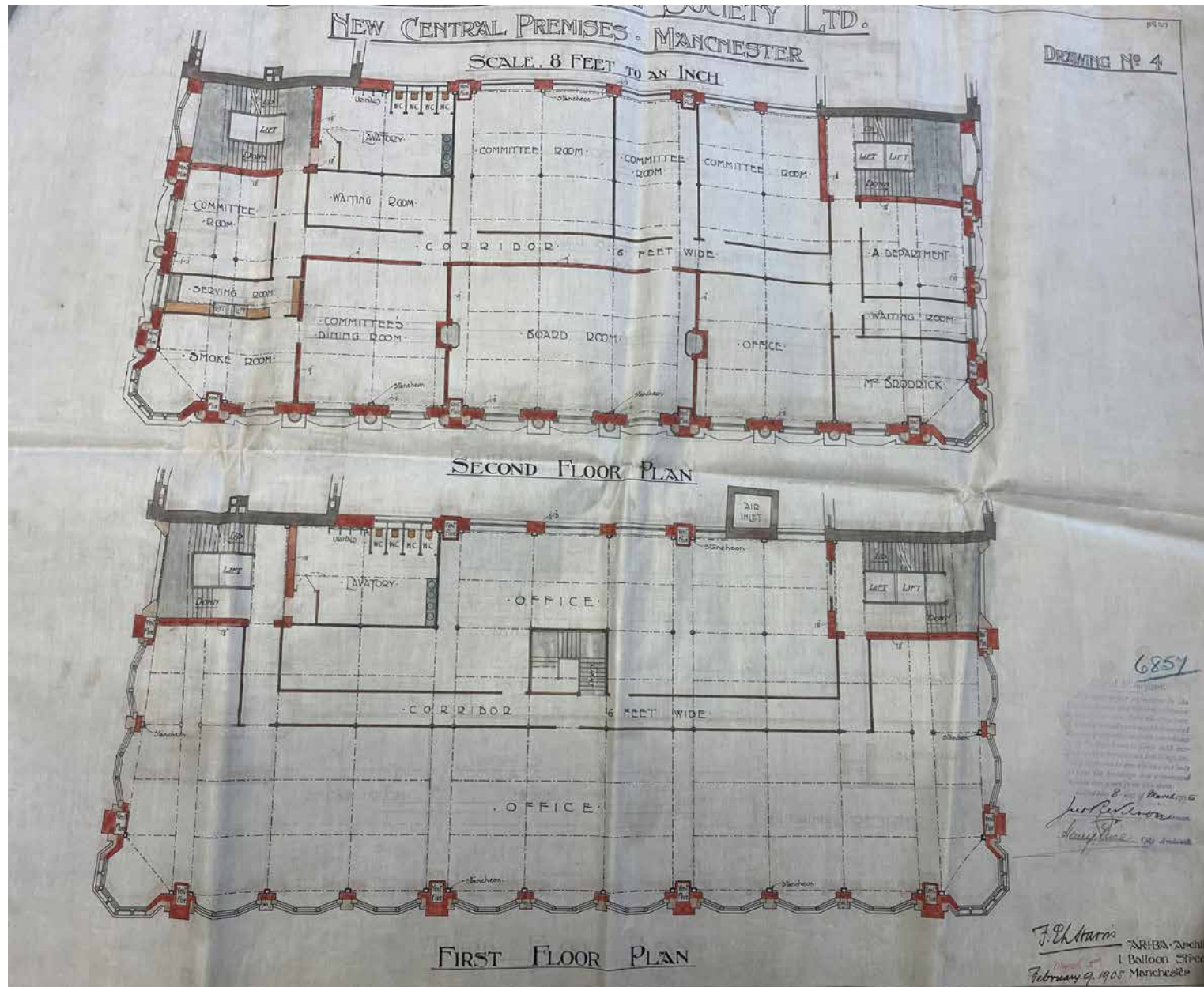
2.20 1905 proposed Hanover House first and second-floor plans (Manchester Archives)
