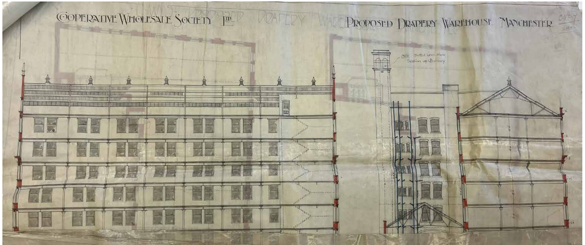
2.6 1901 proposed E block section drawings (Manchester Archives)
