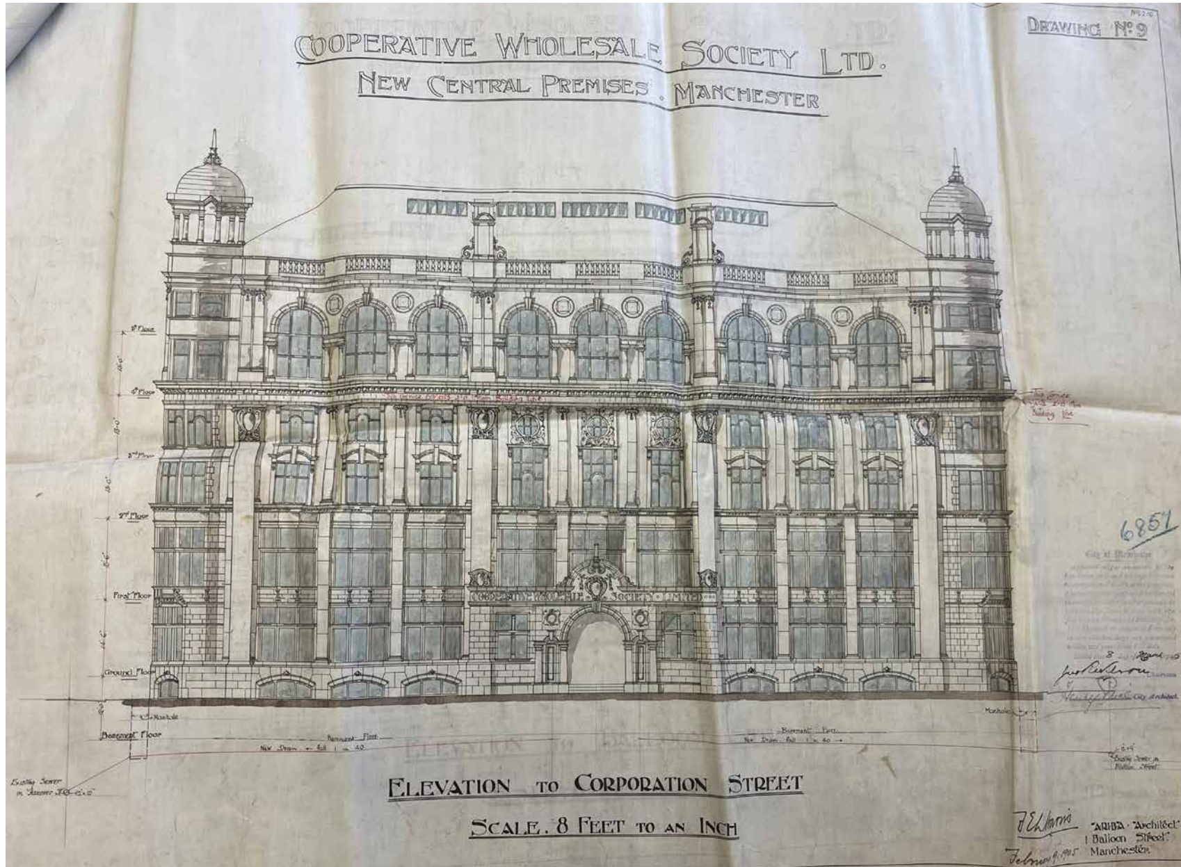
2.12 1905 proposed Hanover House elevation to Corporation Street (Manchester Archives)
