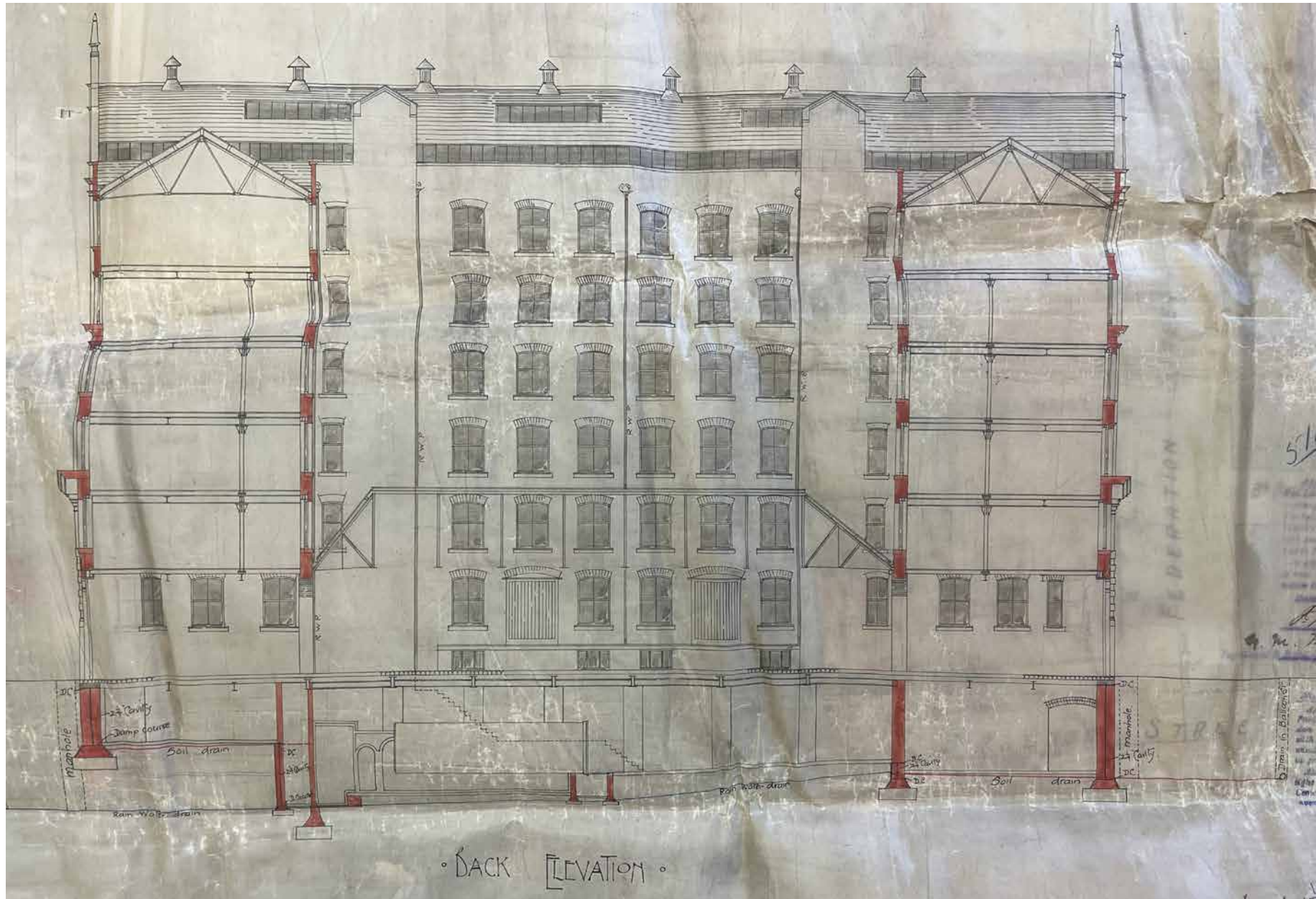
2.5 1901 proposed E block rear elevation (Manchester Archives)
