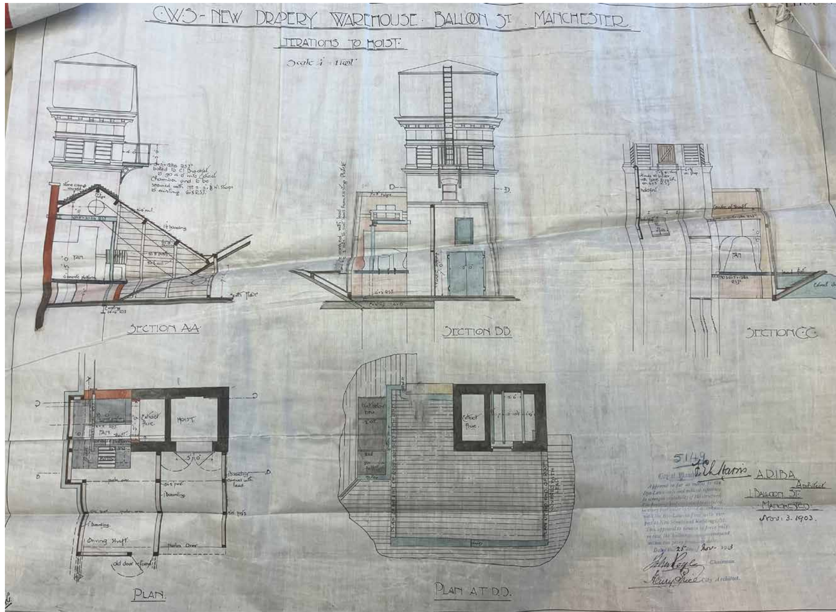
2.10 1903 drawings of the E block tower and hoist (Manchester Archives)
