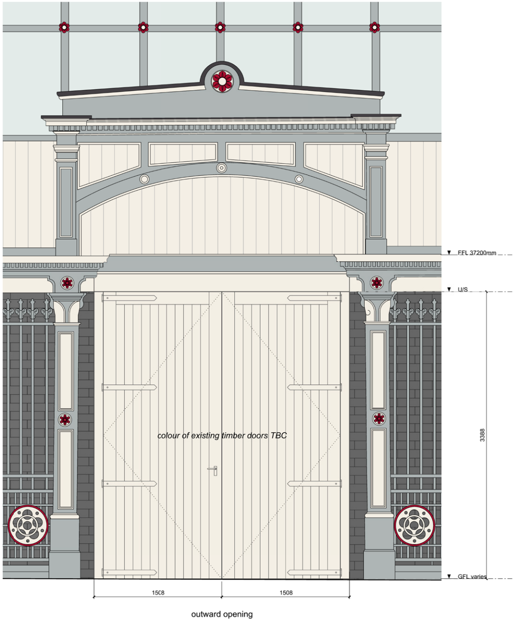
Lower Byrom Street Existing Timber Doors Refurbished Doors Closed
