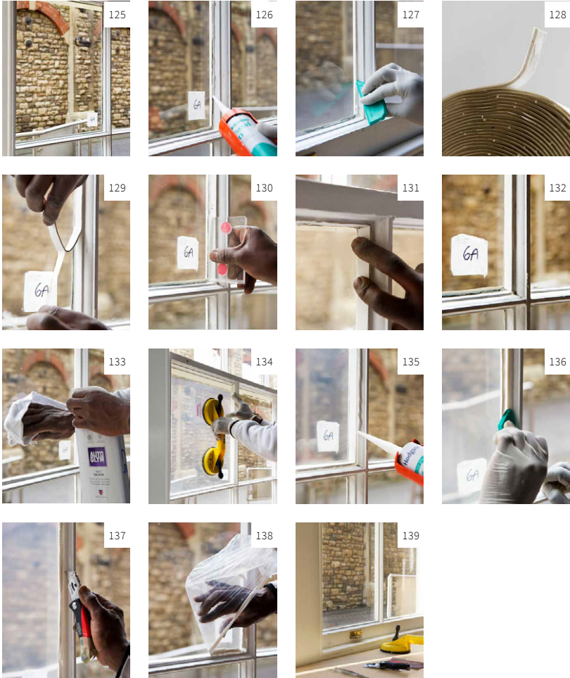
Images 125-139 125-139. This sequence shows the addition of precision cut acrylic glazing to small paned windows. This allows the existing glazing to remain in place The edges need to be carefully sealed to prevent moisture entering the cavity. This is backed up with a specially developed dessicant material inserted in the cavity to prevent condensation.
