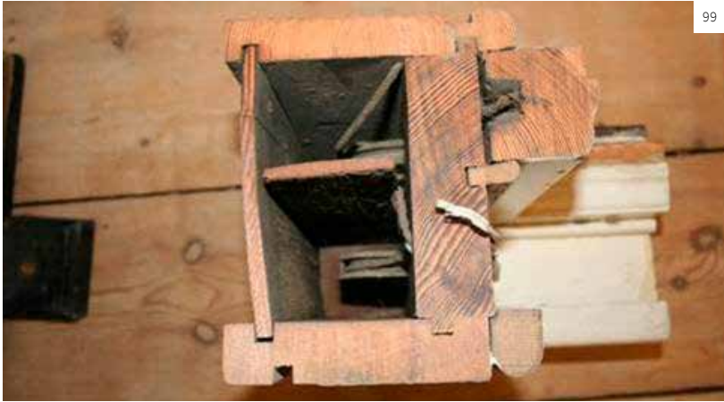
Image 99 This section through a sash box shows the high quality of the timber used during the 19th century.
