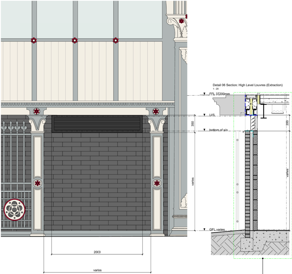
Detail 06: High Level Louvres (Extraction) 1:20
