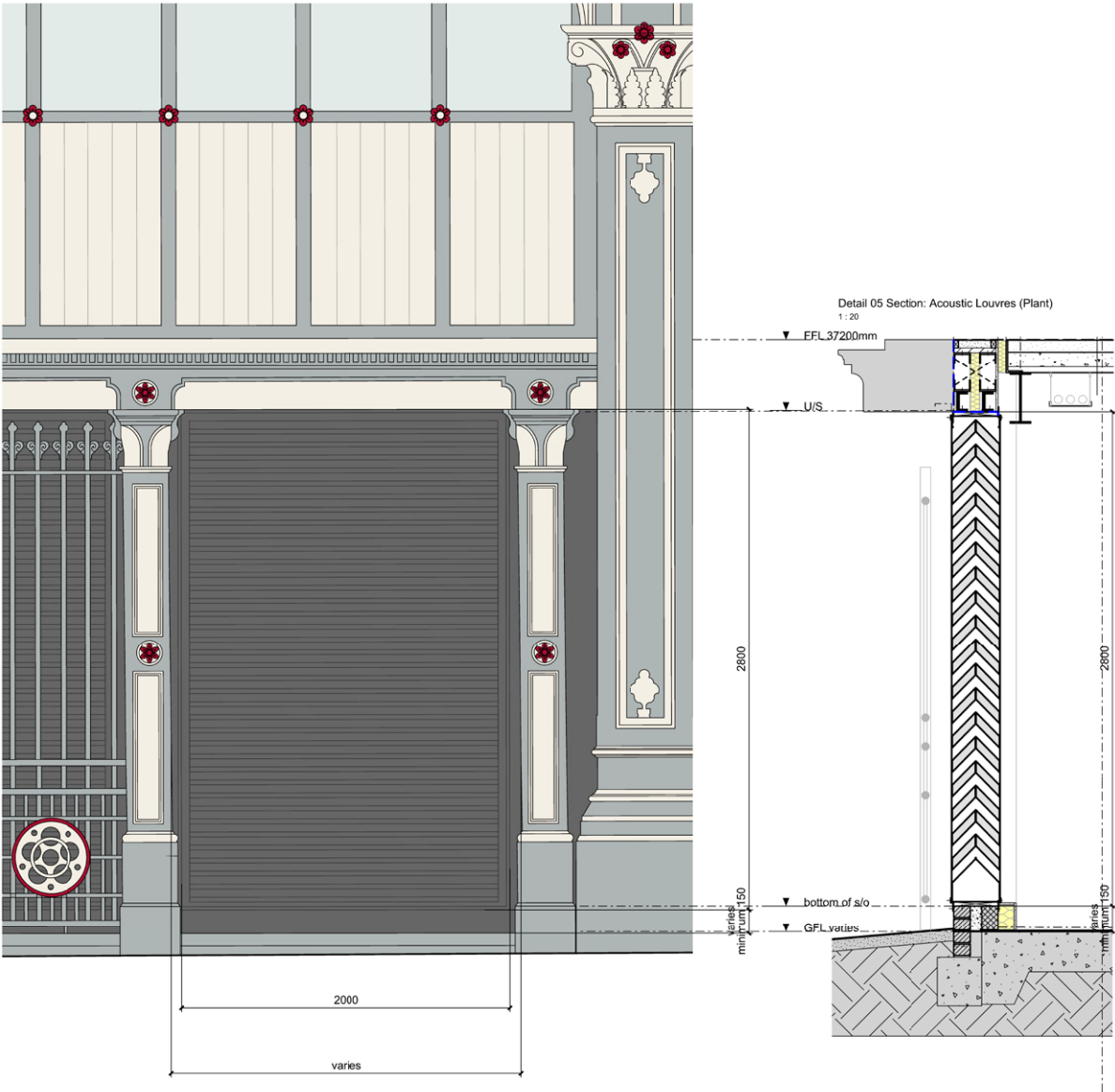
Detail 05: Acoustic Louvres (Plant) 1 : 20
