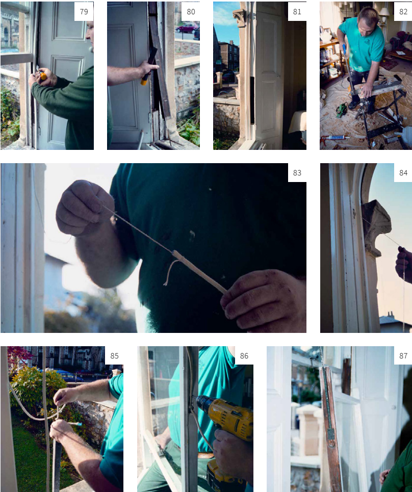
Images 79-87 Replacing a sash cord and adjusting window operation. 79. Removing the staff bead to free the lower sash. 80. Opening the sash pocket. 81. Accessing the weights. 82. Adjusting the weight as necessary to balance the sash. 83. Tying a lead 'mouse' and string to the new sash cord. 84. Running the mouse over the pulley into the weight box. 85. Knotting the weight to the new sash cord. 86. Fixing the cords to the grooves in the sides of the sash. 87. Chains are replaced in much the same way being screwed into the special fitting in the sash.
