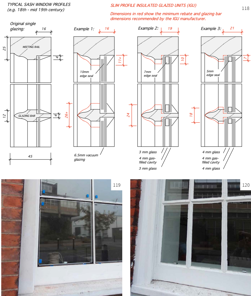
Images 118-120 118. This drawing shows the different thicknesses of insulated glass units currently available when applied to a window with slim glazing bars (Dimensions shown are in millimetres). 119-120. These existing windows had IGUs fitted but the width of the edge seals necessitated the painting of the glazing bars to be extended over the glass so that the seals are not visible.
