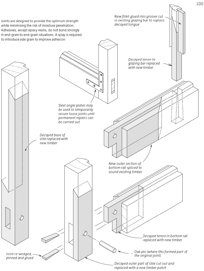
Image 100 Typical timber-to-timber repairs to sash and casement components.
