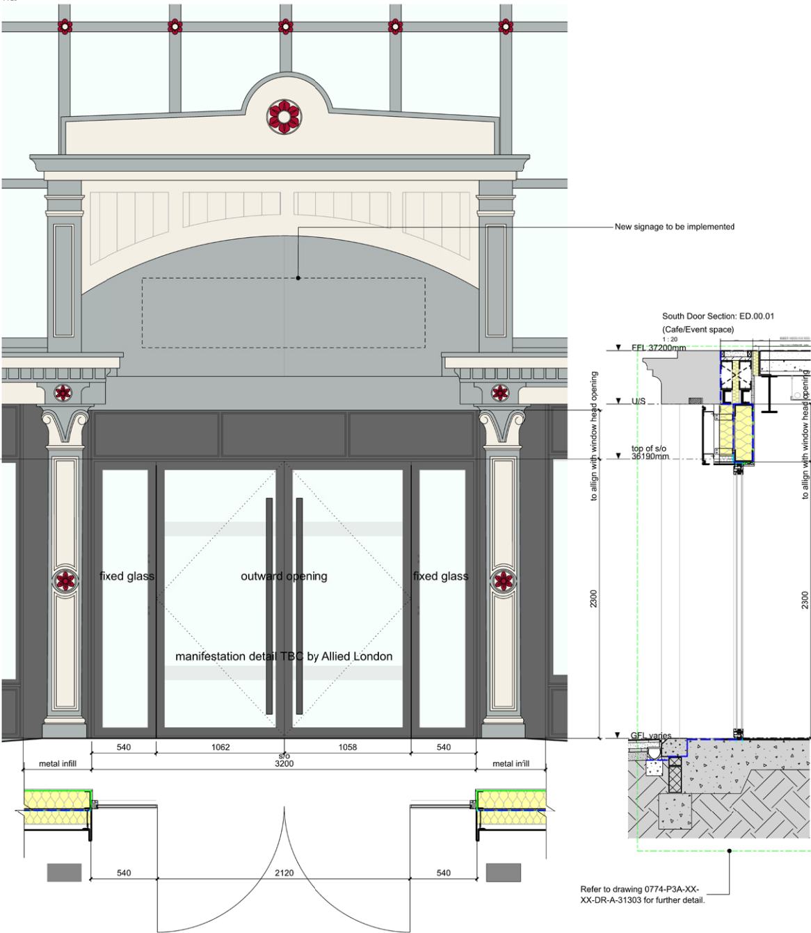
South Door: ED.00.01 (Cafe/ Event Space) 1:20
