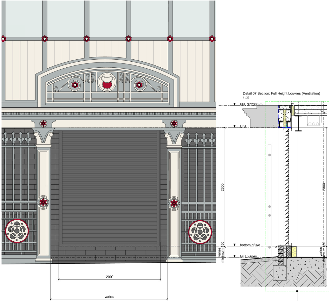
Detail 07: Full Height Louvres (Ventilation) 1:20
