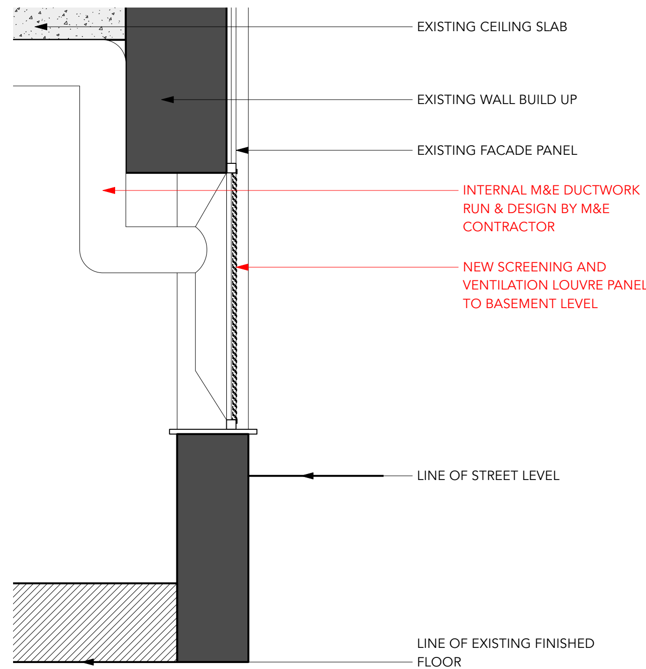
4 ARTILLERY ST FACADE - TYPICAL WINDOW SECTION - PROPOSED Scale: 1:20
