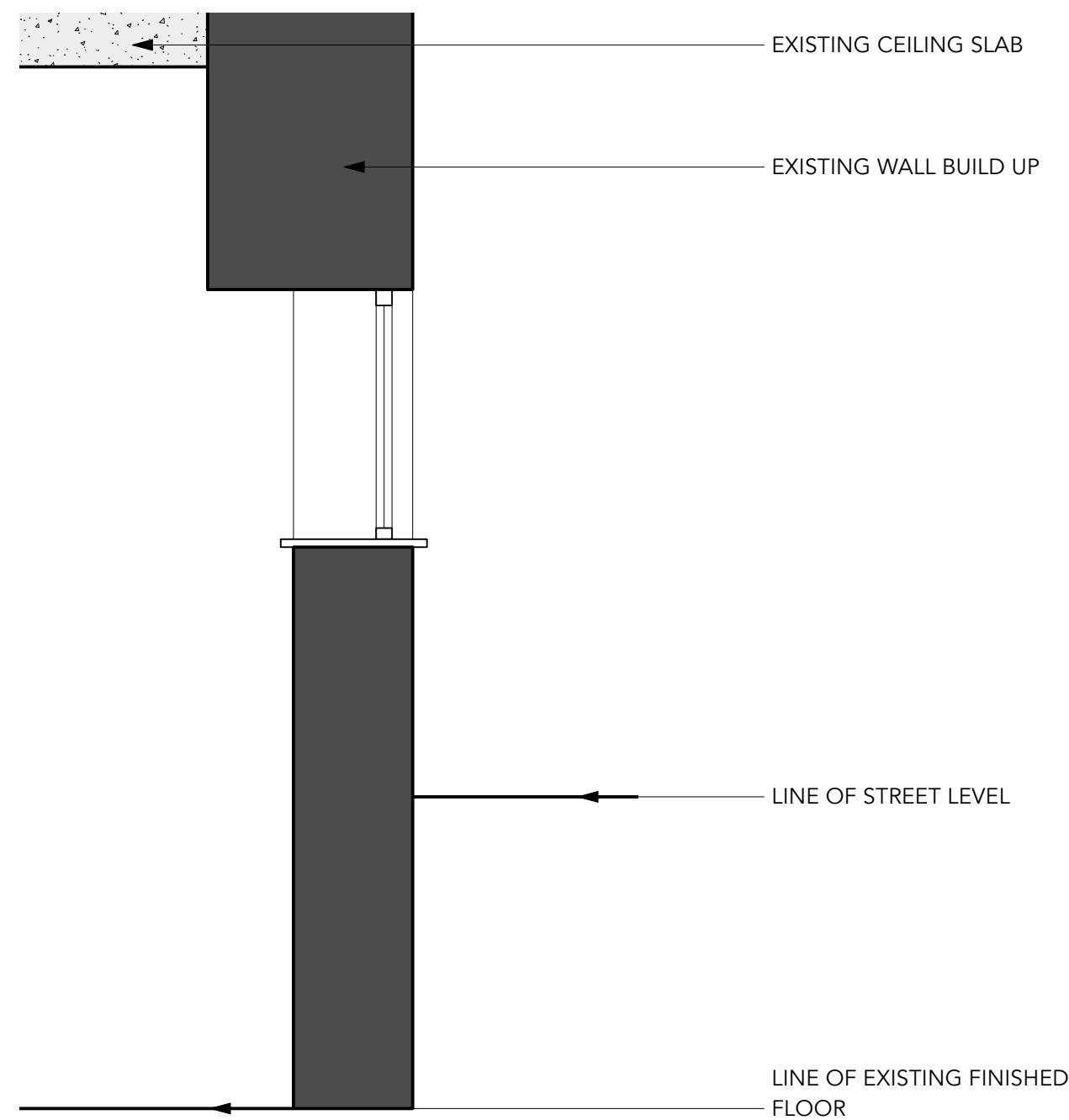
1 ARTILLERY ST FACADE - TYPICAL WINDOW SECTION - EXISTING Scale: 1:20
