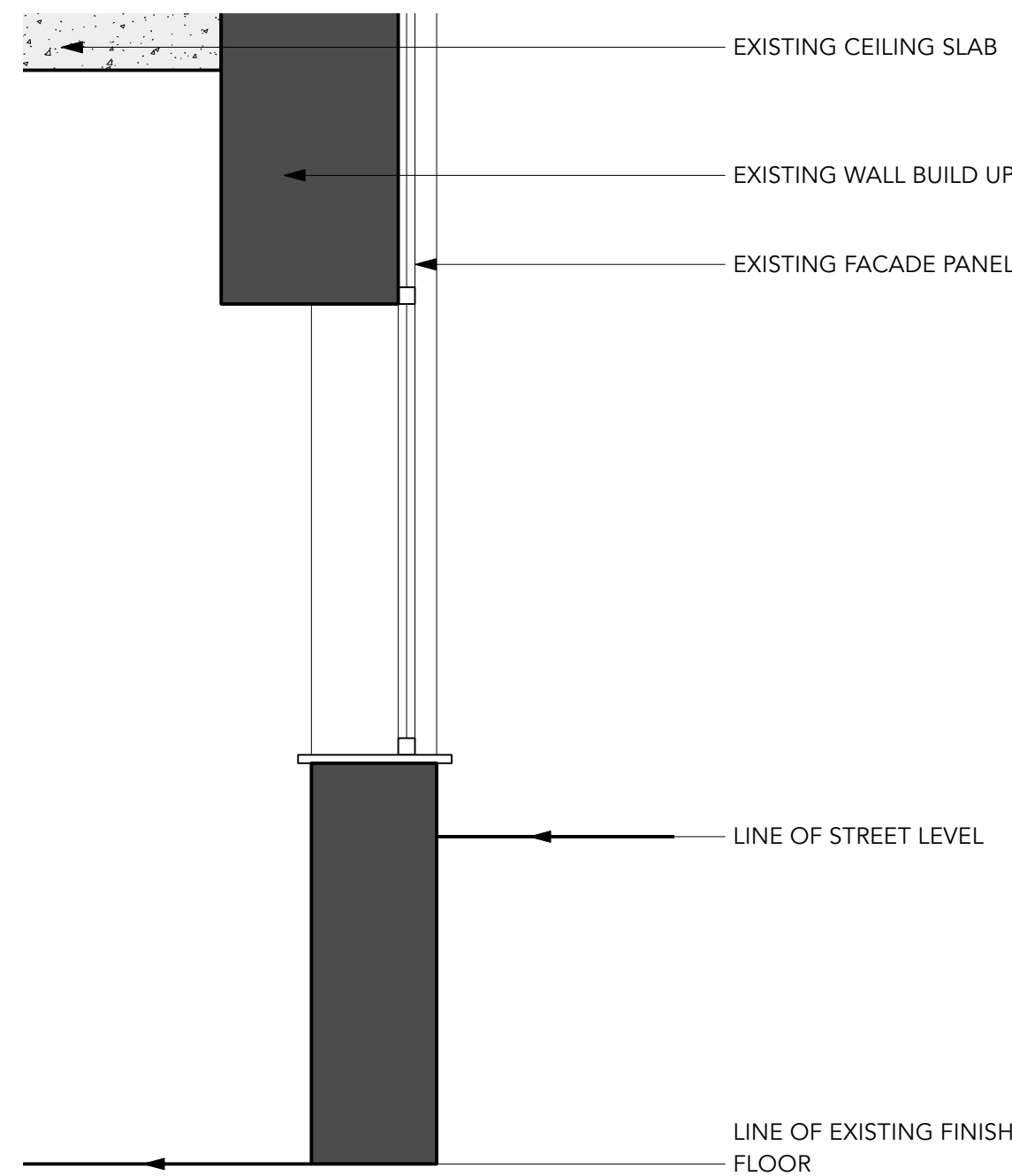
3 ARTILLERY ST FACADE - TYPICAL WINDOW SECTION - EXISTING Scale: 1:20
