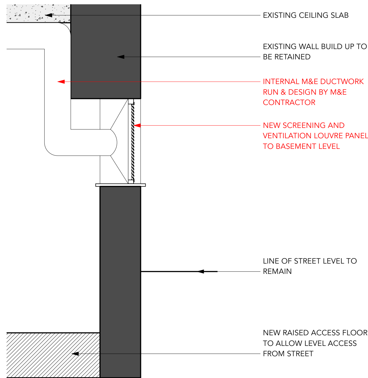
2 ARTILLERY ST FACADE - TYPICAL WINDOW SECTION - PROPOSED Scale: 1:20
