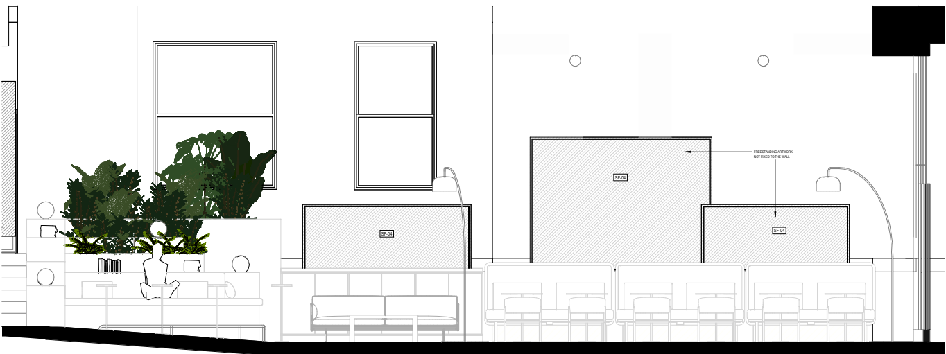
GROUND FLOOR ELEVATION - ATRIUM - EAST WALL SOUTH PORTION 1:25
