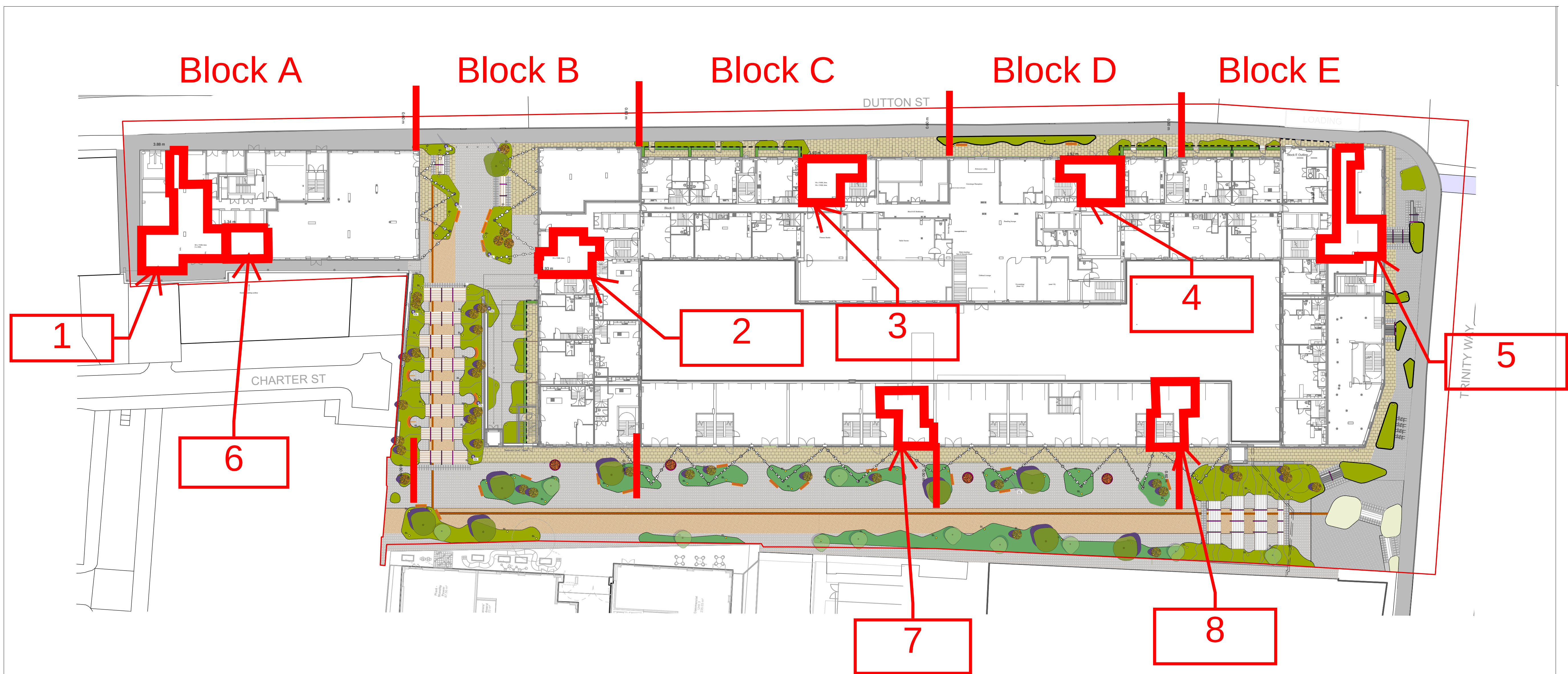
1 General Arrangement Scale: 1:350
