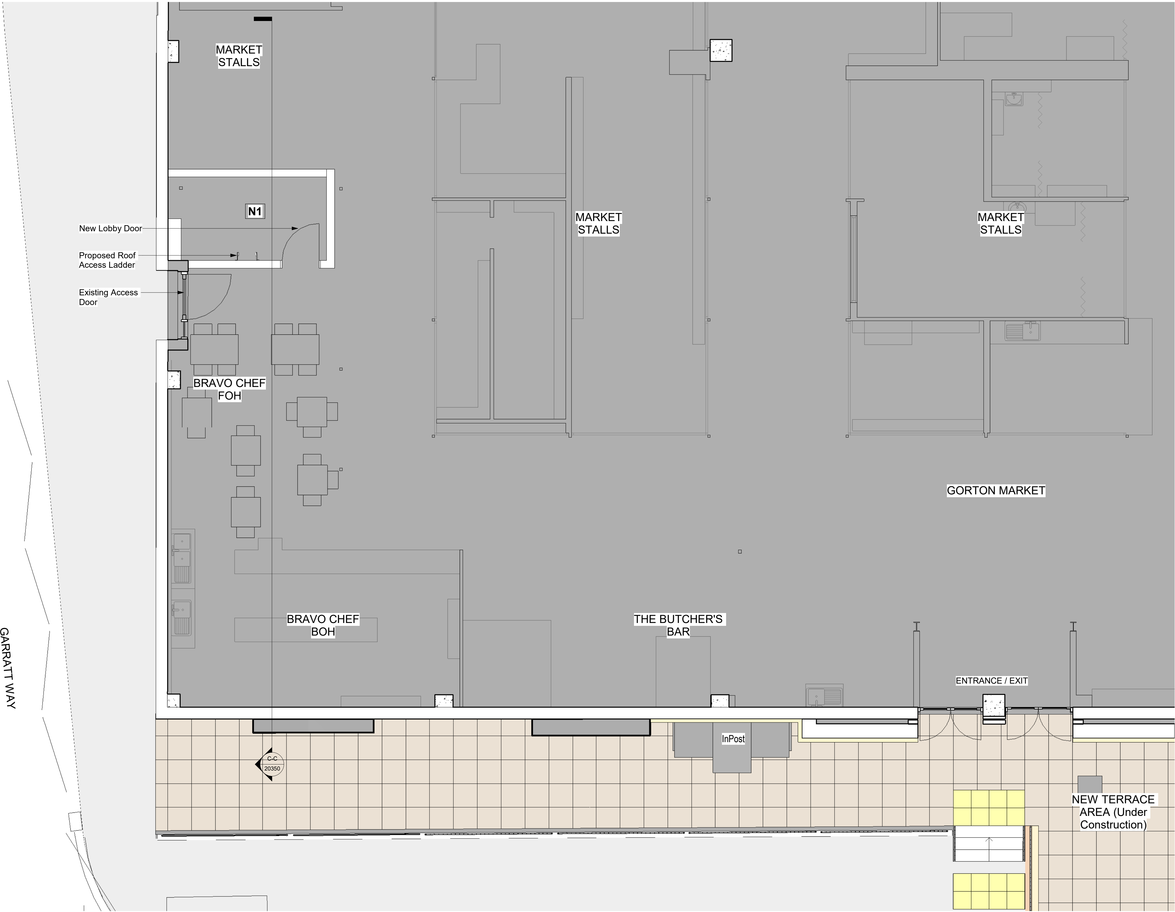
Proposed Roof Access Lobby Plan
