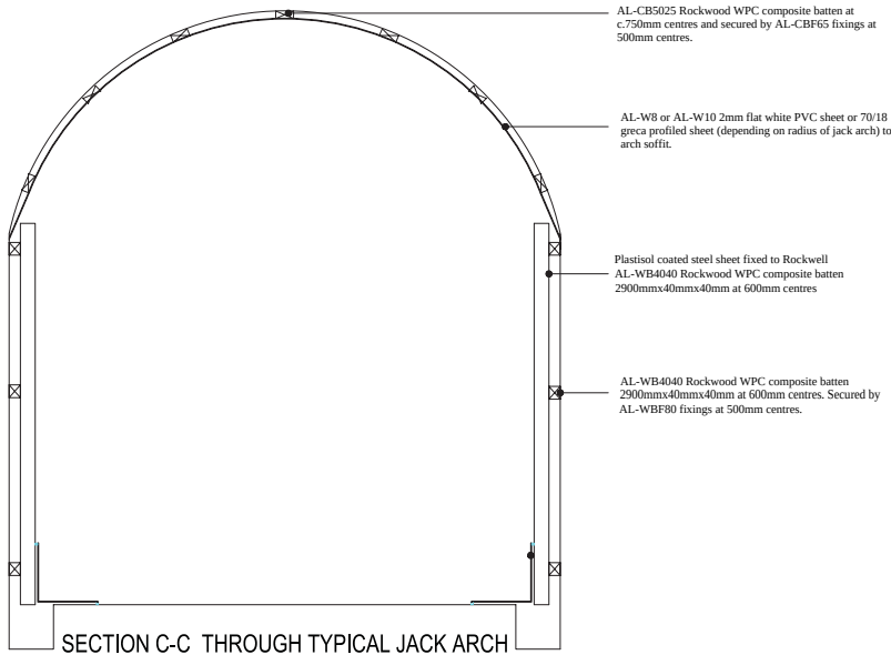
SECTION C-C THROUGH TYPICAL JACK ARCH
