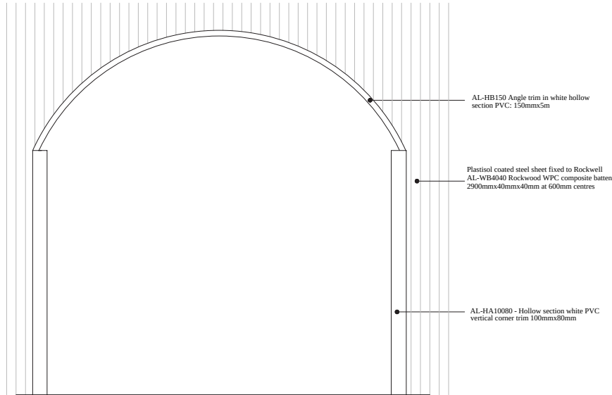
TYPICAL JACK ARCH ELEVATION
