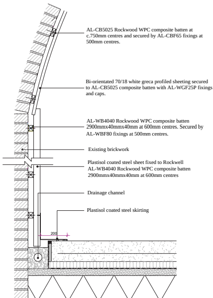
SECTION THROUGH TYPICAL ARCH WALL
