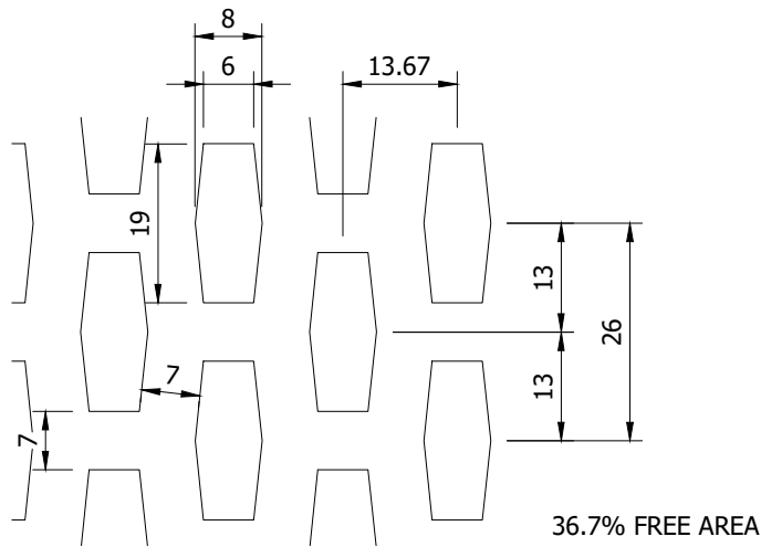
DT4 PERFORATION DETAIL SCALE - 1:4
