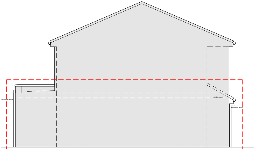
PROPOSED R/H SIDE PARTY WALL ELEVATION
