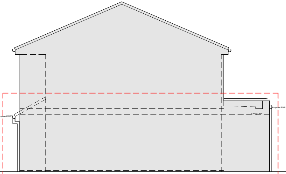
PROPOSED R/H SIDE PARTY WALL ELEVATION
